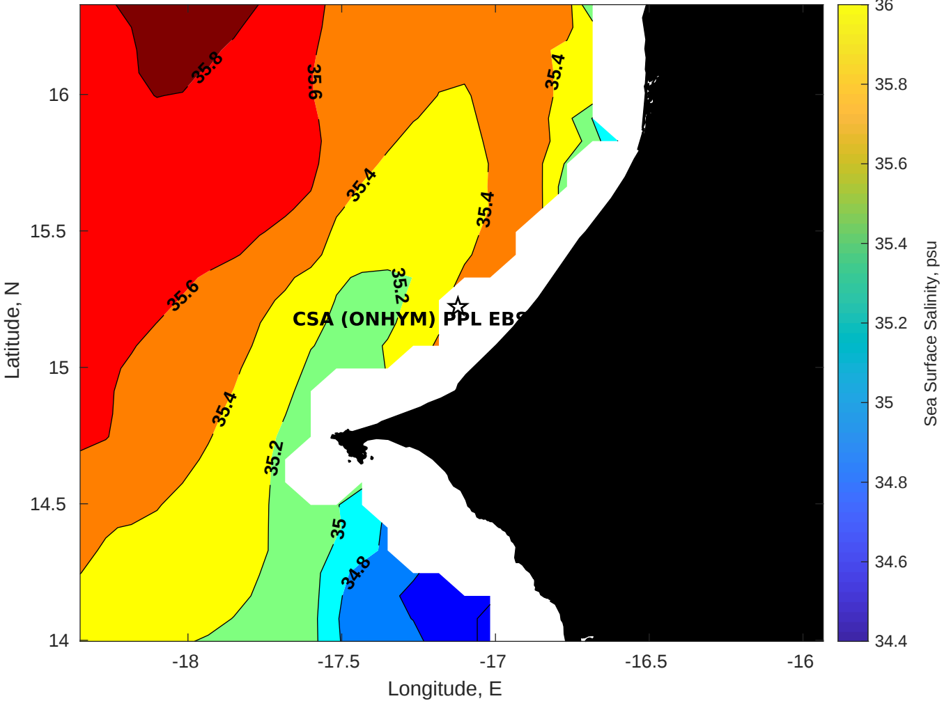
Surface Salinity for CSA (ONHYM) PPL EBS - Senegal at 09-Oct-2025 00:00:00
