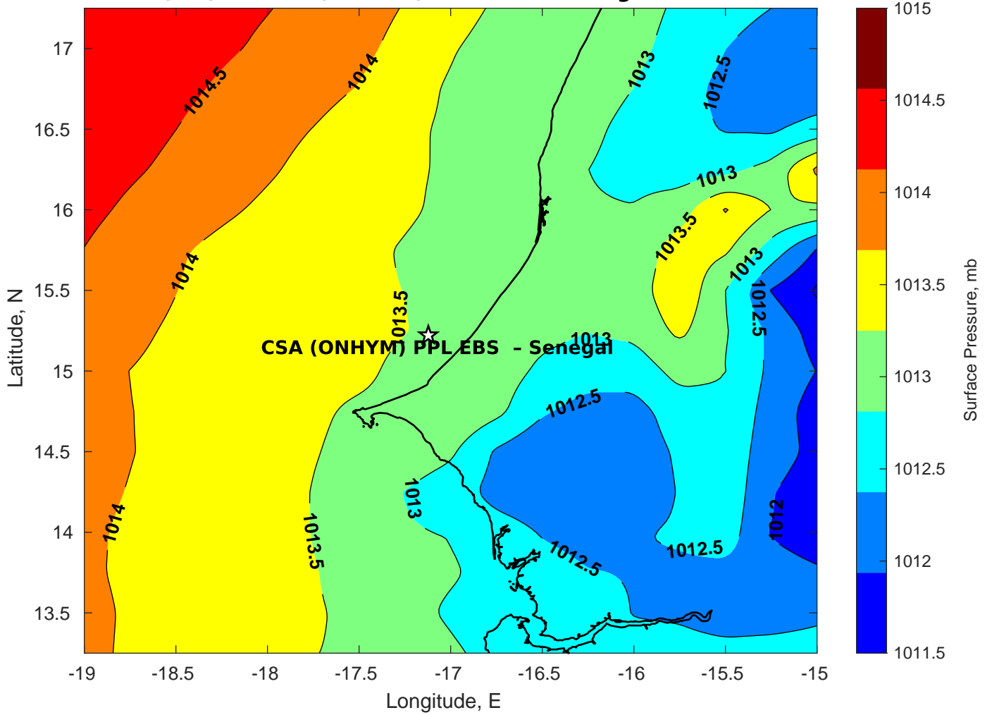
Surface Pressure (mb) for CSA (ONHYM) PPL EBS - Senegal at 10-Oct-2025 00:00:00
