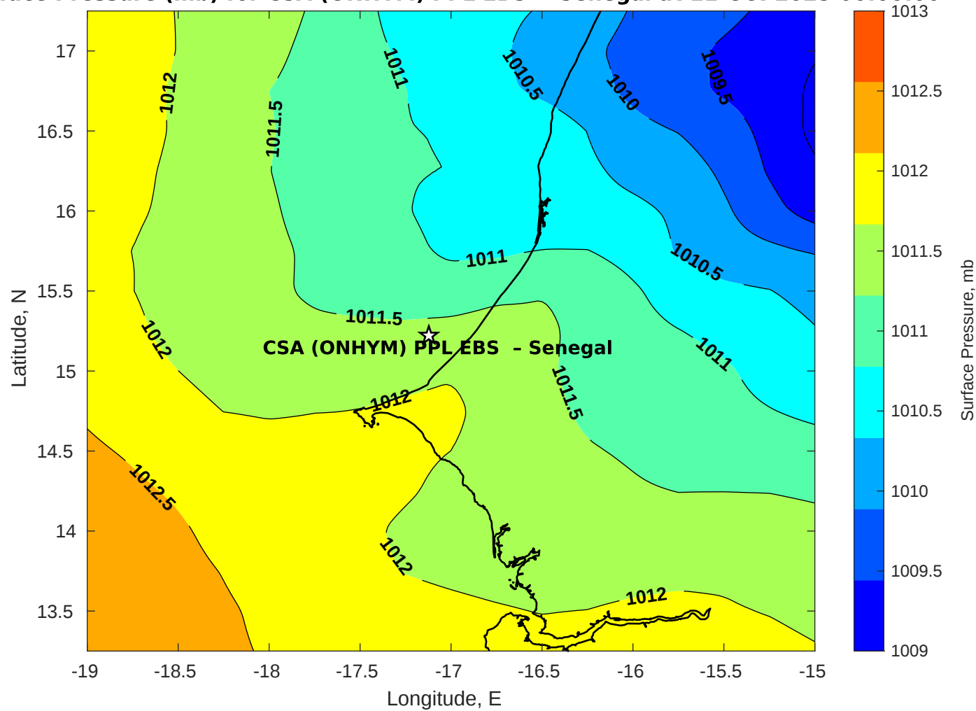
Surface Pressure (mb) for CSA (ONHYM) PPL EBS - Senegal at 11-Oct-2025 00:00:00
