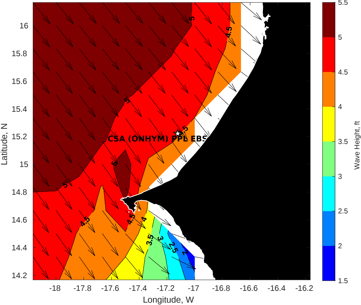
Wave Height (ft) for CSA (ONHYM) PPL EBS - Senegal at 10-Oct-2025 09:00:00
