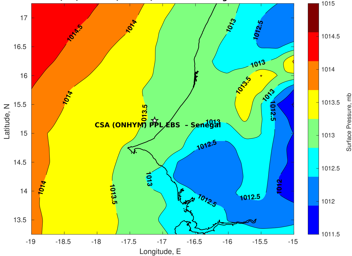
Surface Pressure (mb) for CSA (ONHYM) PPL EBS - Senegal at 10-Oct-2025 00:00:00
