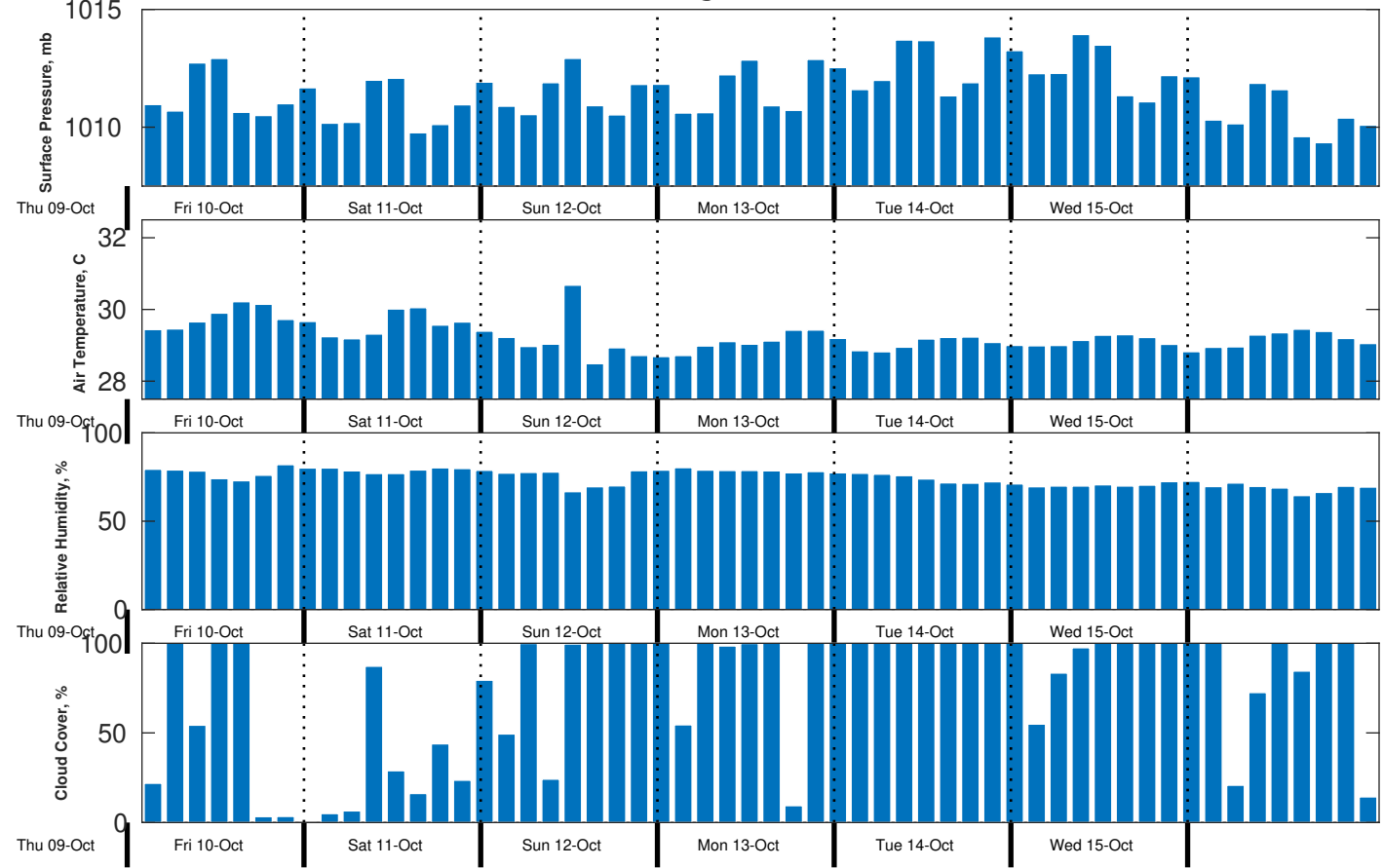
Met Forecast for CSA (ONHYM) PPL EBS - Senegal from 10-Oct-2025 00:00:00 to 17-Oct-2025 00:00:00
