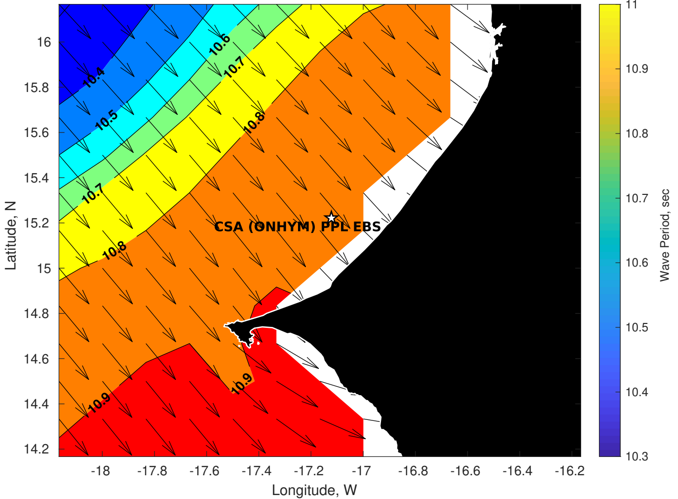
Wave Period (sec) for CSA (ONHYM) PPL EBS - Senegal at 10-Oct-2025 09:00:00
