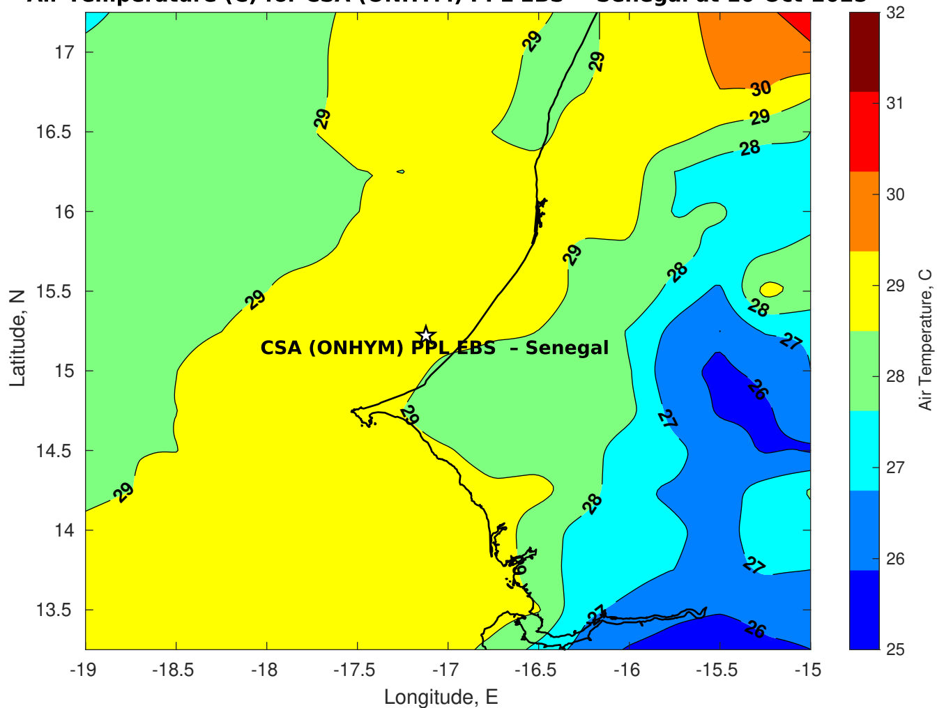
Air Temperature (C) for CSA (ONHYM) PPL EBS - Senegal at 10-Oct-2025
