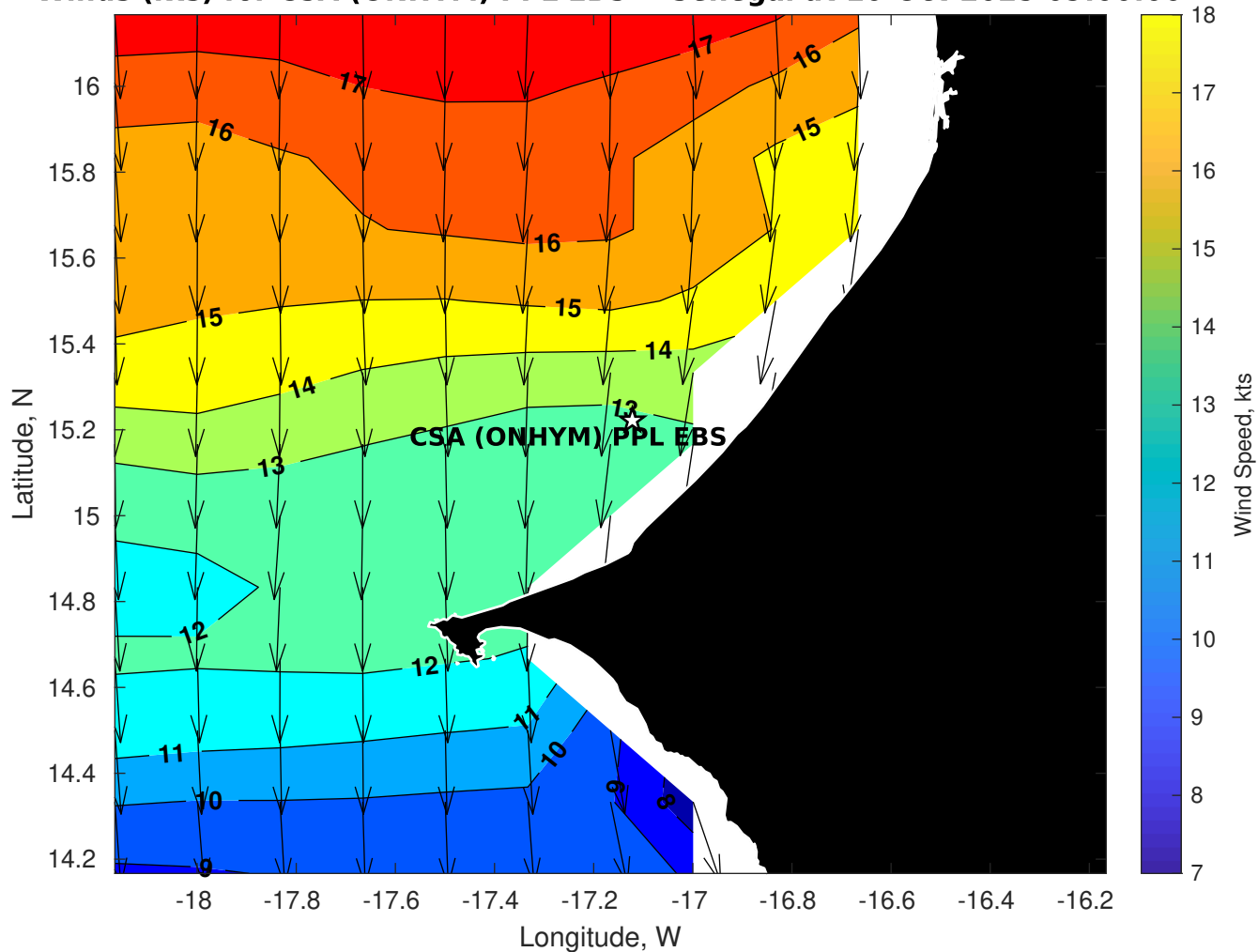
Winds (kts) for CSA (ONHYM) PPL EBS - Senegal at 10-Oct-2025 09:00:00
