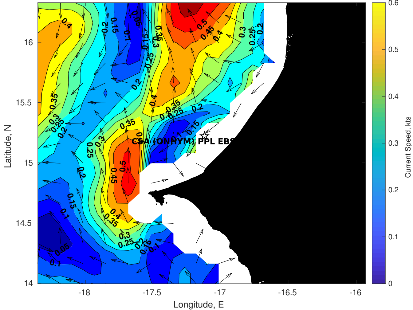
Surface Currents for CSA (ONHYM) PPL EBS - Senegal at 09-Oct-2025 00:00:00
