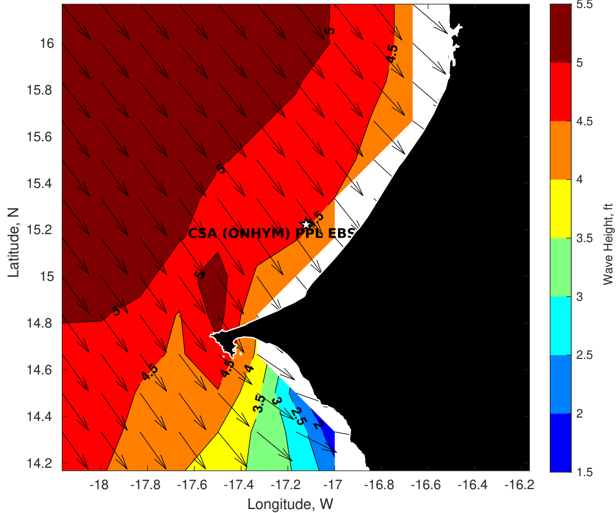
Wave Height (ft) for CSA (ONHYM) PPL EBS - Senegal at 10-Oct-2025 09:00:00
