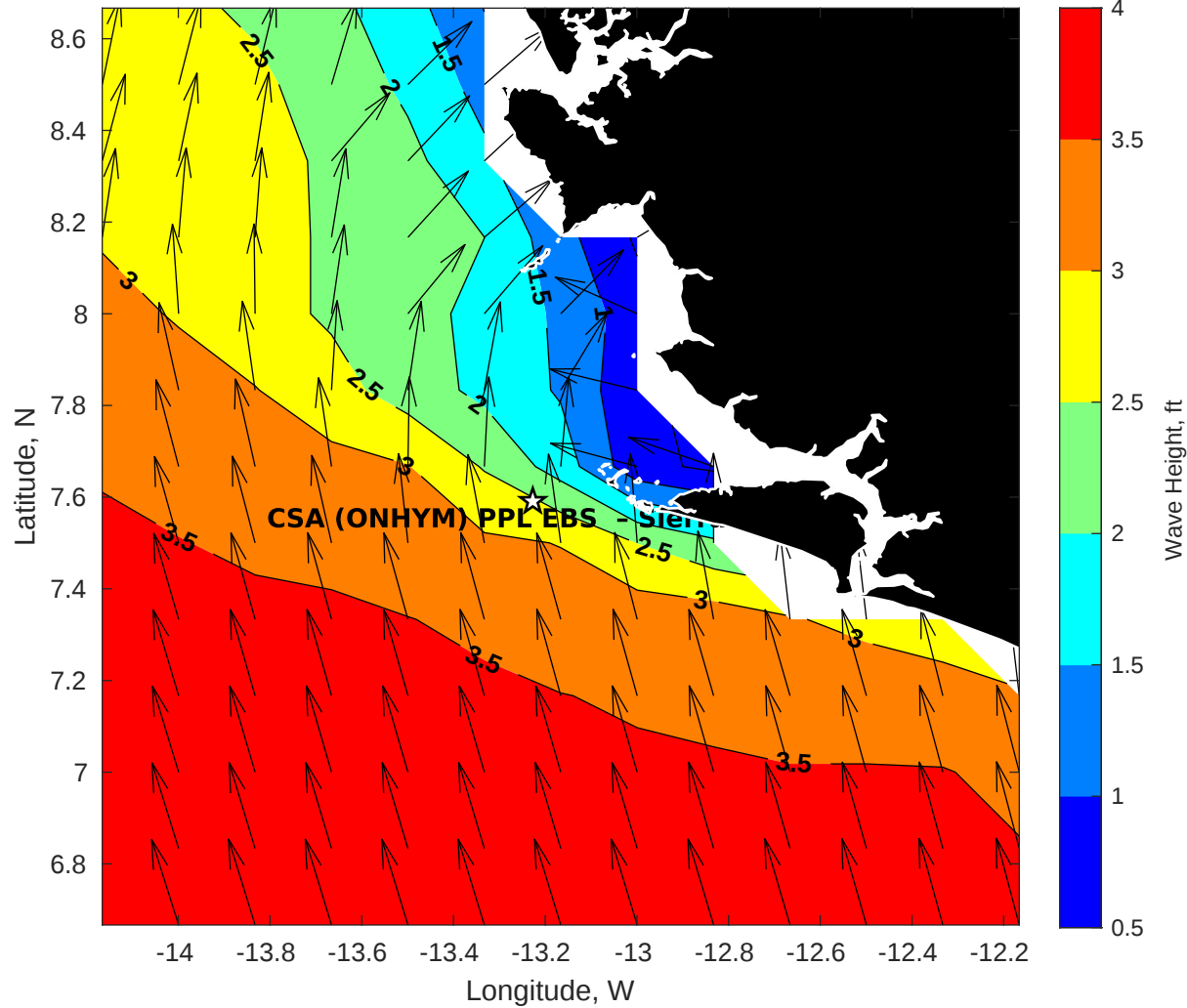
Wave Height (ft) for CSA (ONHYM) PPL EBS - Sierra Leone at 10-Oct-2025 09:00:00
