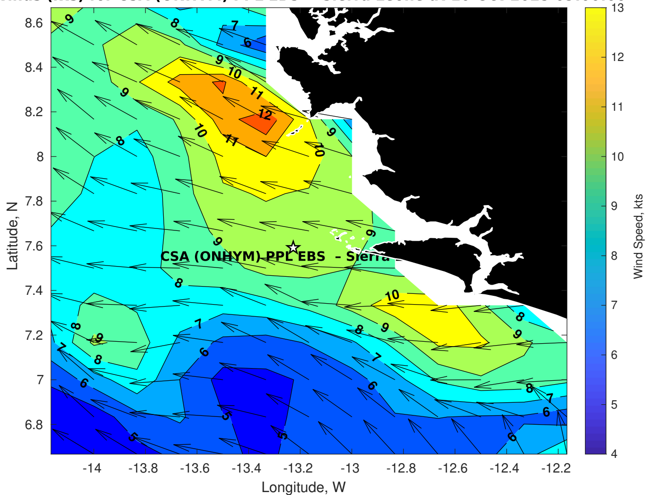
Winds (kts) for CSA (ONHYM) PPL EBS - Sierra Leone at 10-Oct-2025 09:00:00
