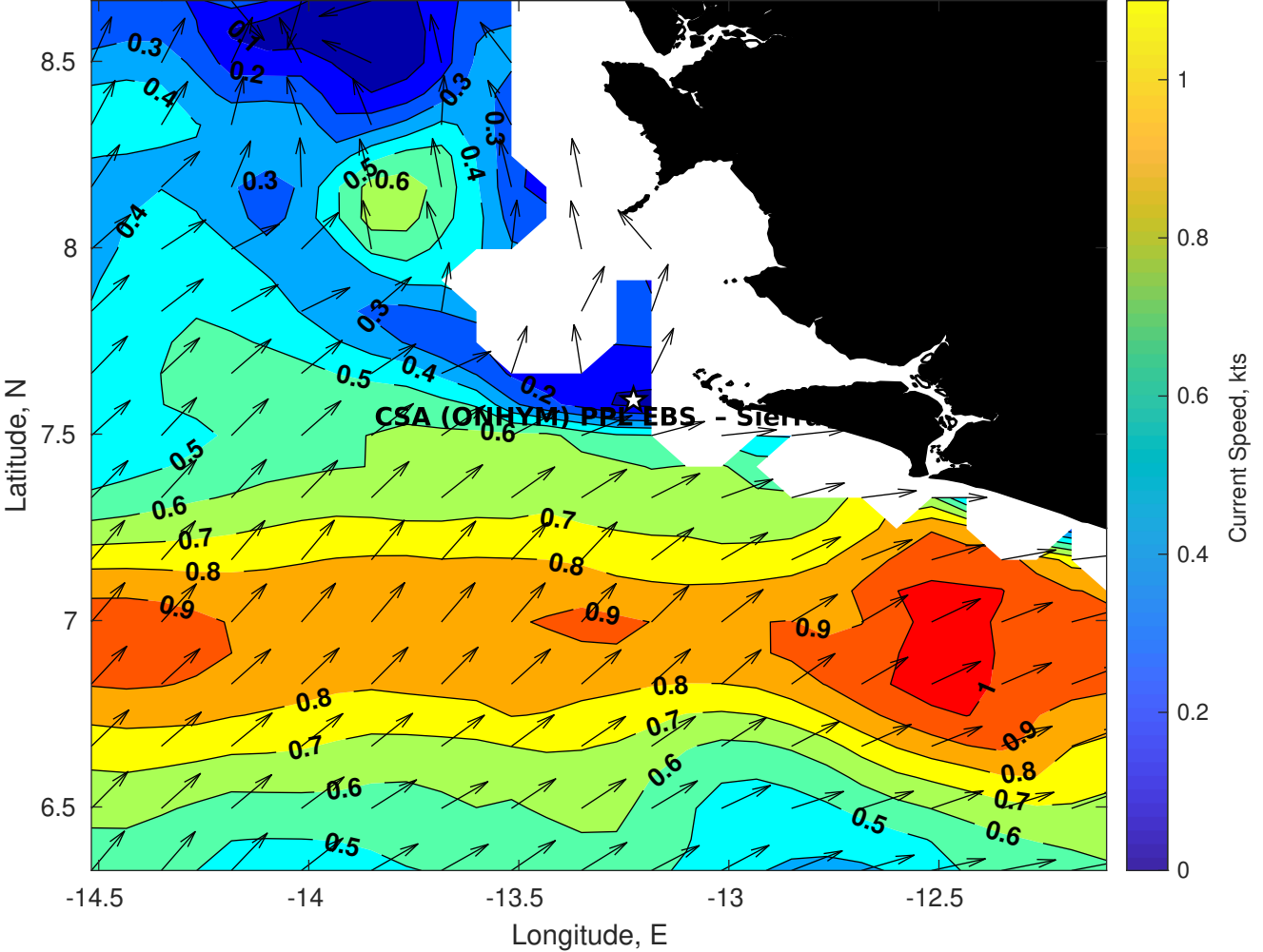
Surface Currents for CSA (ONHYM) PPL EBS - Sierra Leone at 09-Oct-2025 00:00:00
