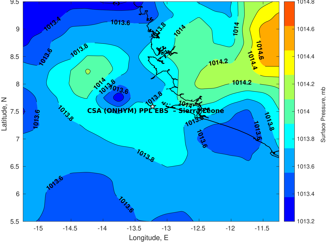
Surface Pressure (mb) for CSA (ONHYM) PPL EBS - Sierra Leone at 10-Oct-2025 00:00:00
