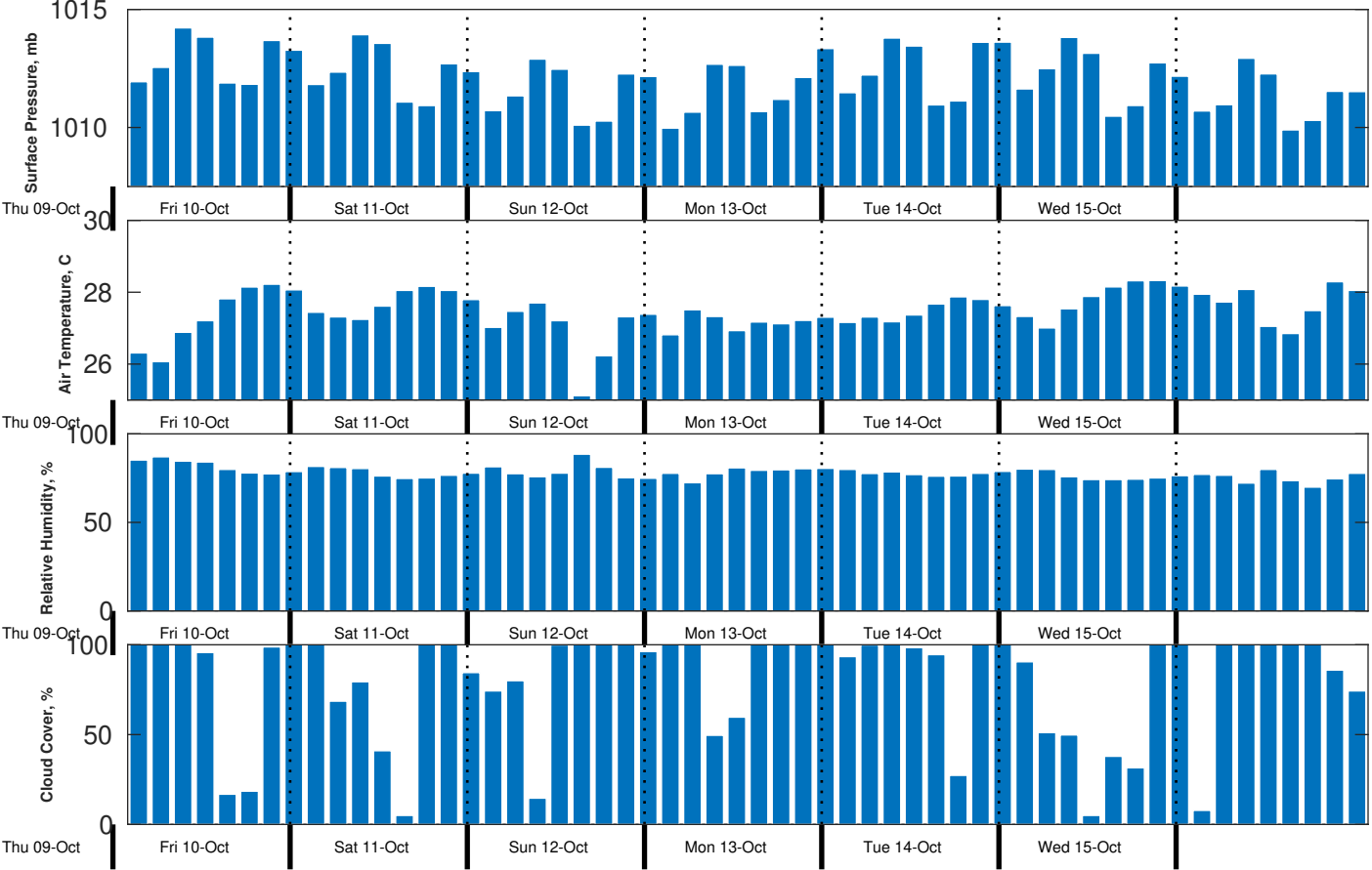
Met Forecast for CSA (ONHYM) PPL EBS - Sierra Leone from 10-Oct-2025 00:00:00 to 17-Oct-2025 00:00:00
