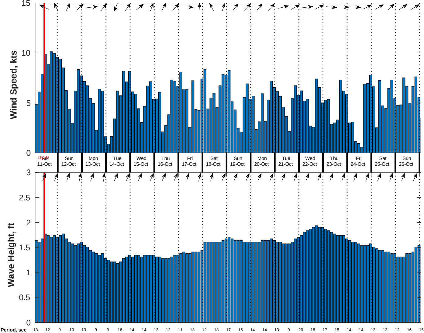
Wind & Wave Forecast for CSA (ONHYM) PPL EBS - Sierra Leone from 10-Oct-2025 01:00:00 to 26-Oct-2025 01:00:00
