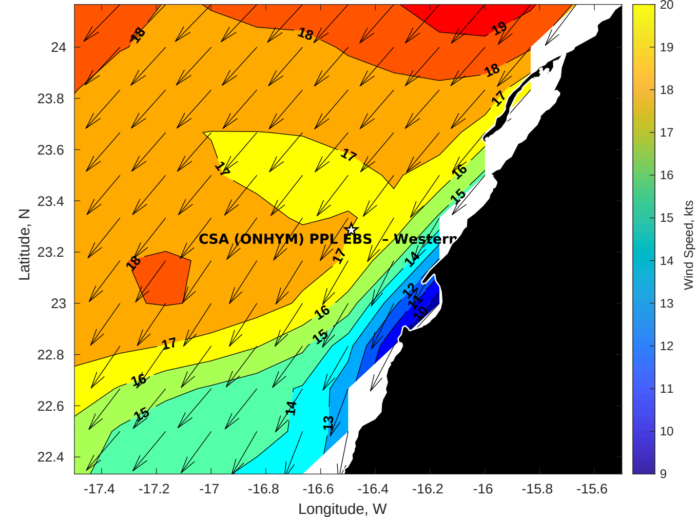
Winds (kts) for CSA (ONHYM) PPL EBS - Western Sahara at 10-Oct-2025 09:00:00
