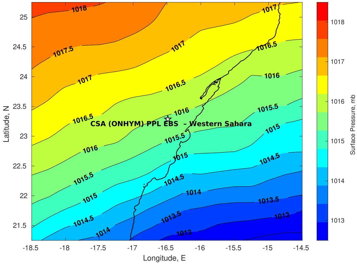
Surface Pressure (mb) for CSA (ONHYM) PPL EBS - Western Sahara at 11-Oct-2025 00:00:00
