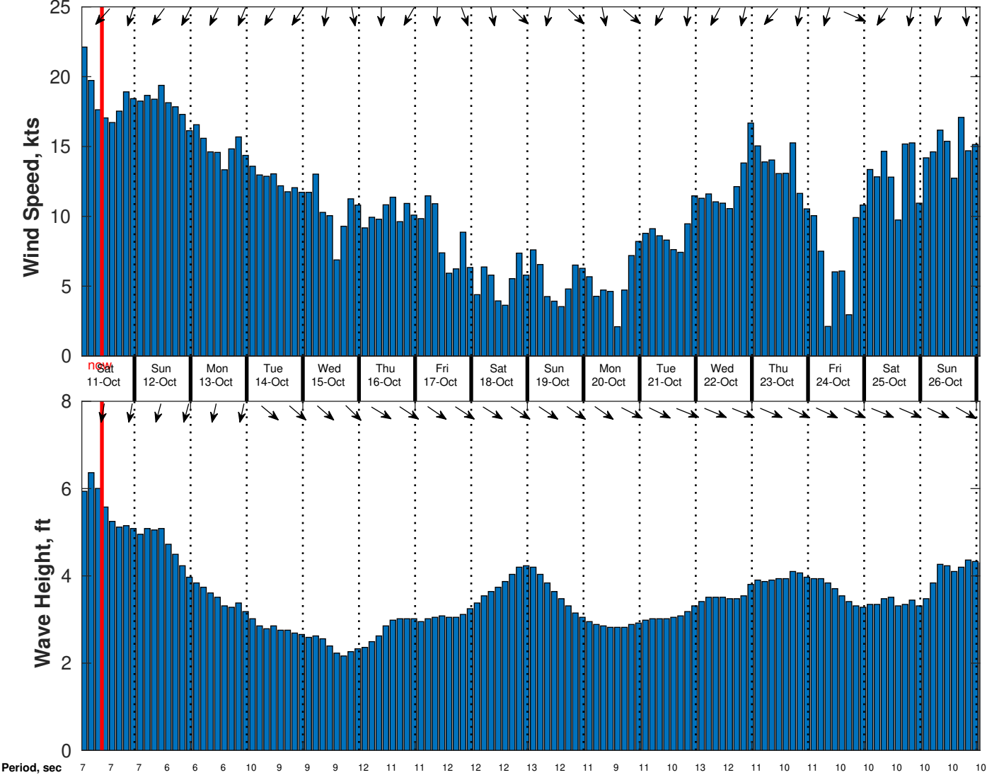
Wind & Wave Forecast for CSA (ONHYM) PPL EBS - Western Sahara from 10-Oct-2025 01:00:00 to 26-Oct-2025 01:00:00
