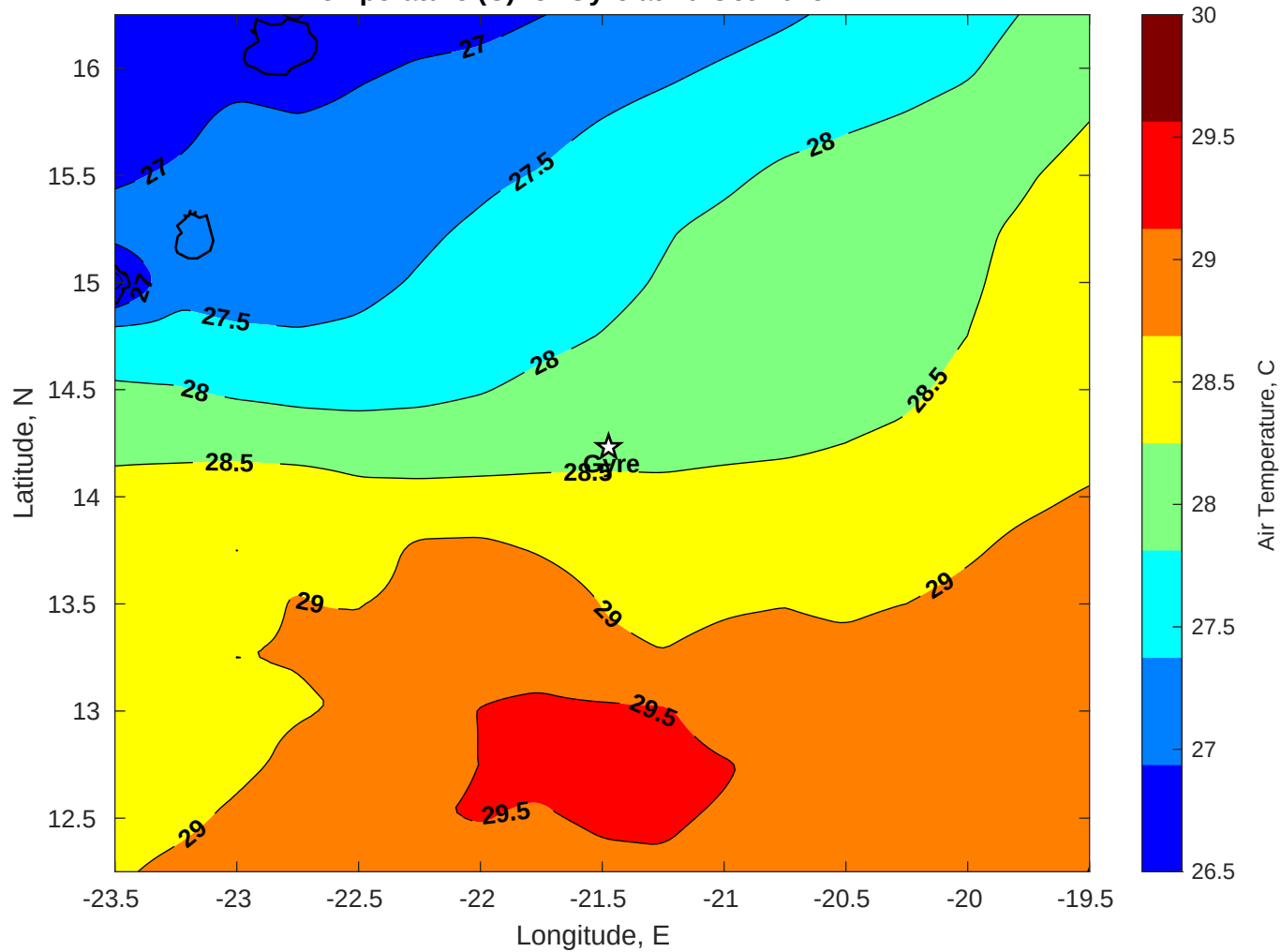
Air Temperature (C) for Gyre at 10-Oct-2025
