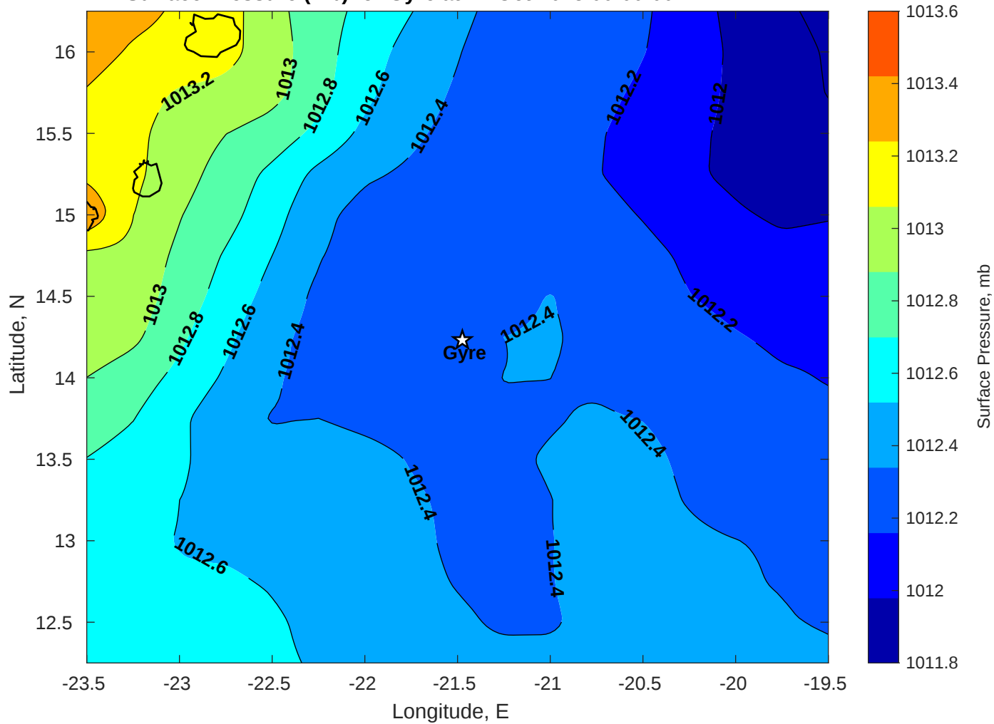
Surface Pressure (mb) for Gyre at 12-Oct-2025 00:00:00
