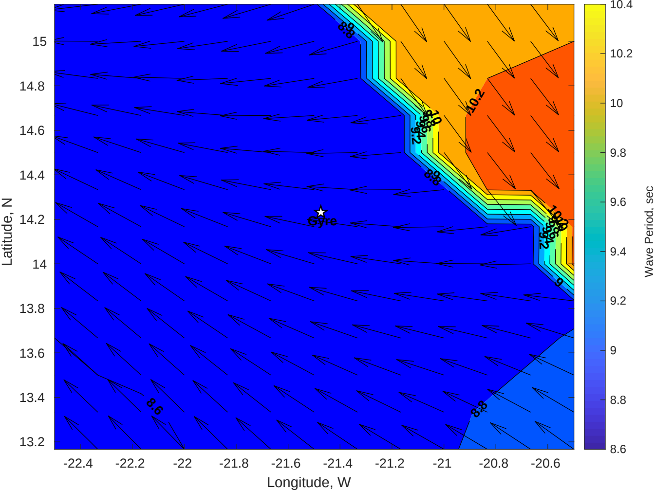
Wave Period (sec) for Gyre at 10-Oct-2025 09:00:00
