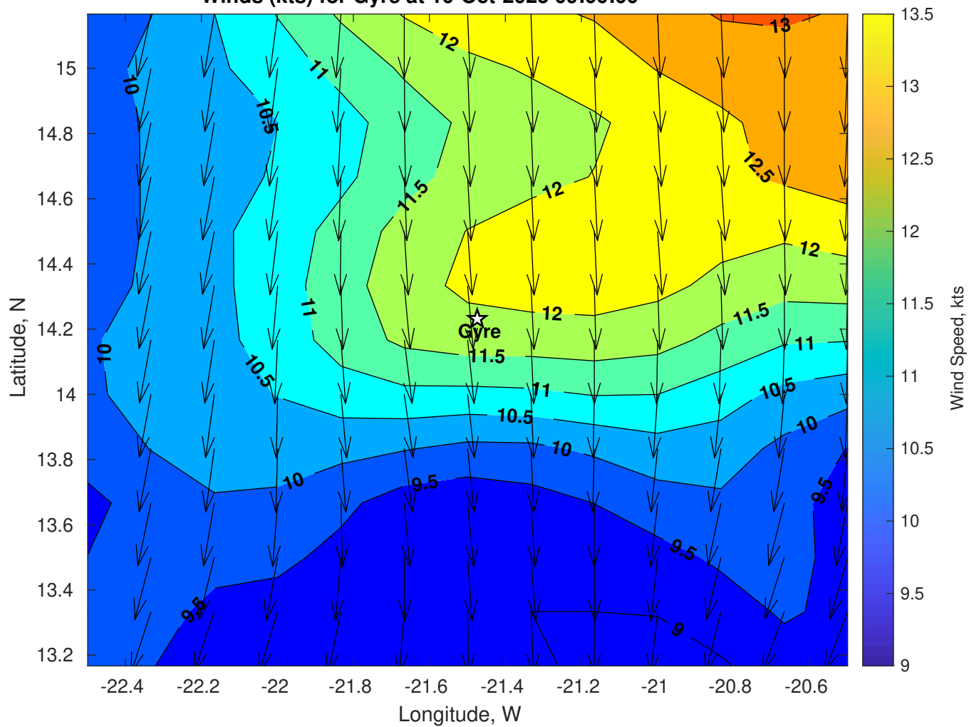
Winds (kts) for Gyre at 10-Oct-2025 09:00:00
