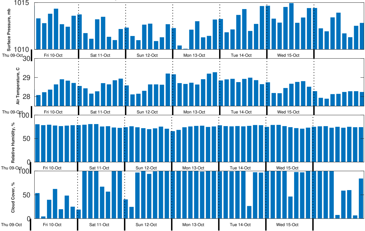
Met Forecast for Gyre from 09-Oct-2025 23:00:00 to 16-Oct-2025 23:00:00
