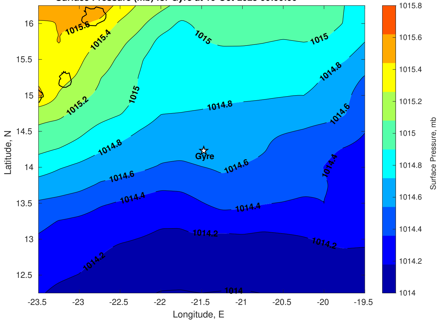
Surface Pressure (mb) for Gyre at 10-Oct-2025 00:00:00
