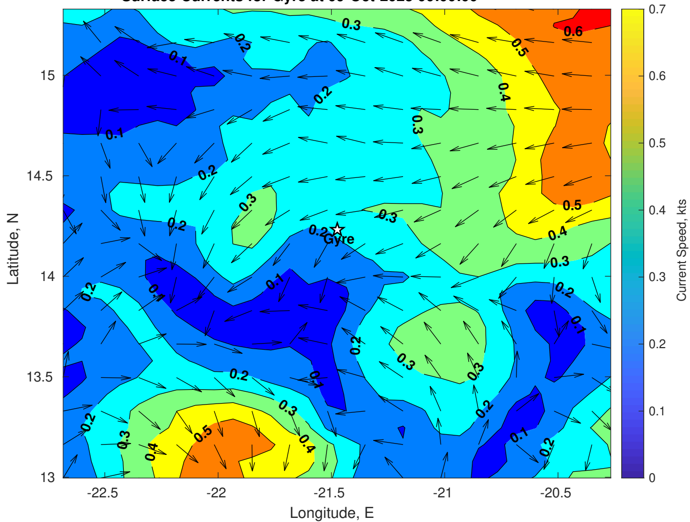
Surface Currents for Gyre at 09-Oct-2025 00:00:00
