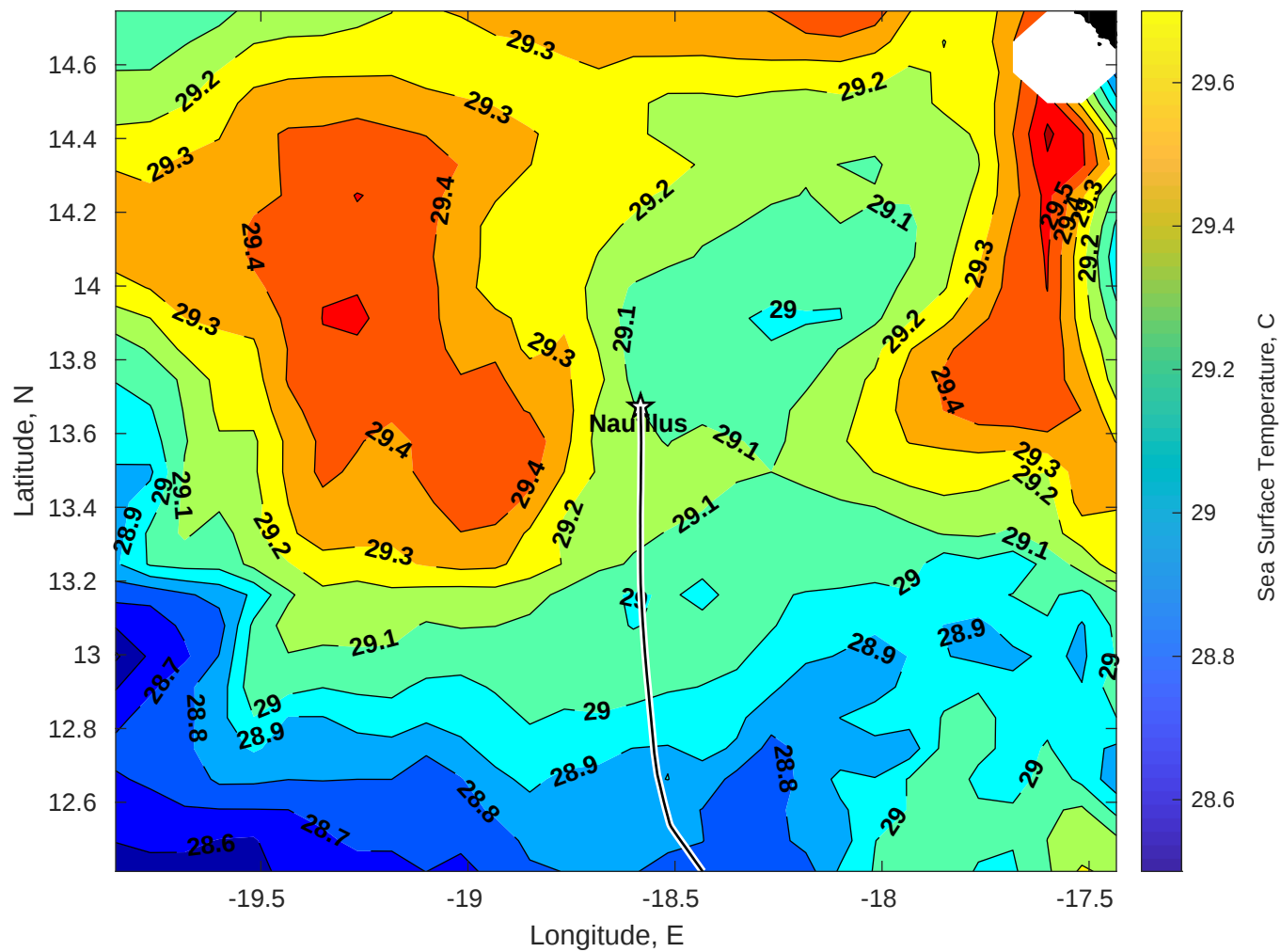
SST for Nautilus at 09-Oct-2025 00:00:00
