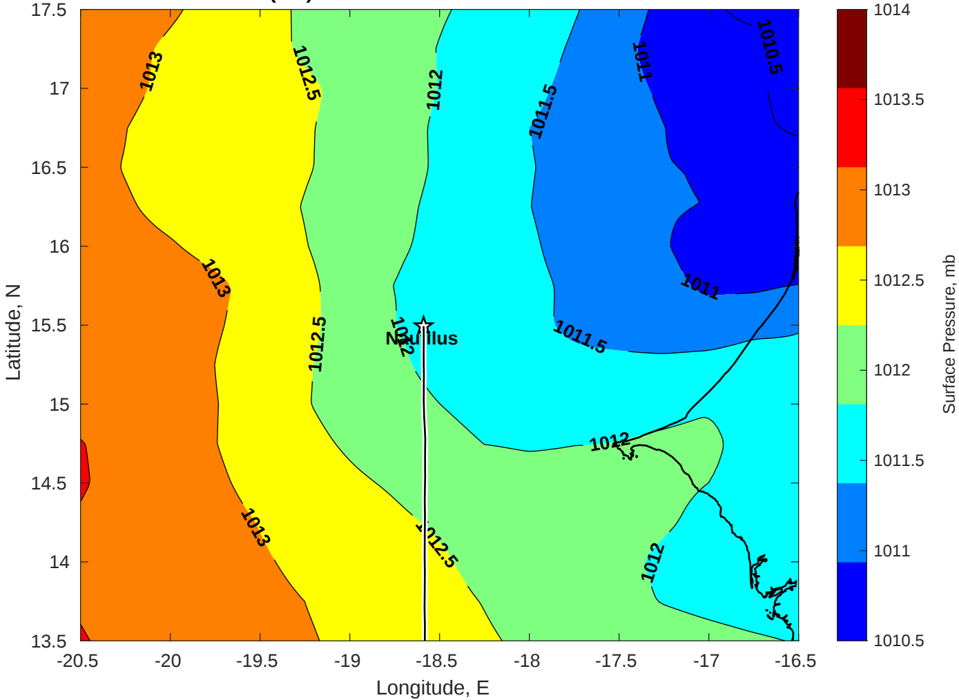
Surface Pressure (mb) for Nautilus at 11-Oct-2025 00:00:00
