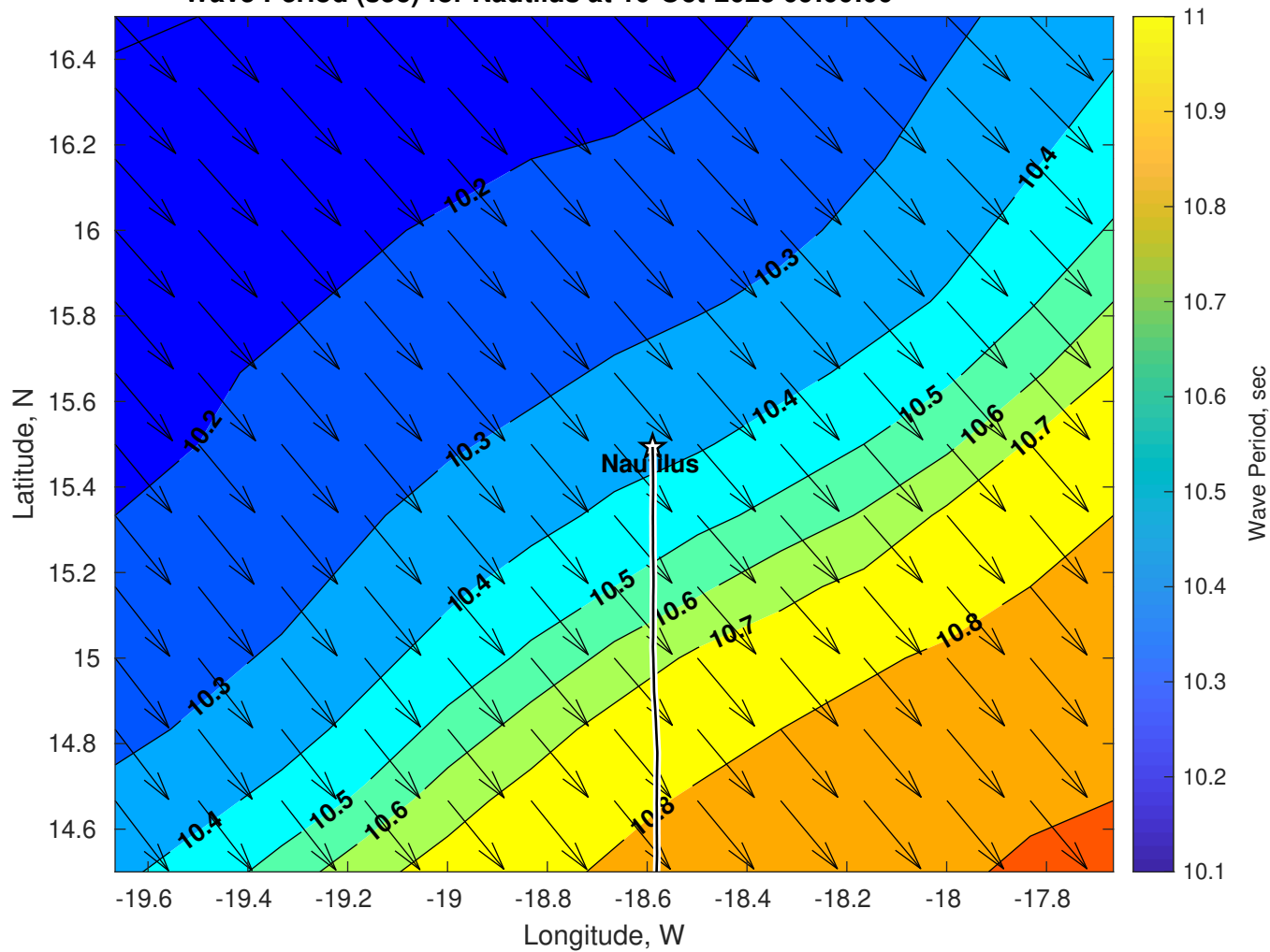
Wave Period (sec) for Nautilus at 10-Oct-2025 09:00:00
