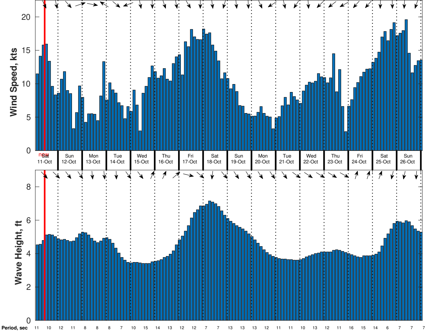
Wind & Wave Forecast for Nautilus from 10-Oct-2025 02:00:00 to 26-Oct-2025 02:00:00
