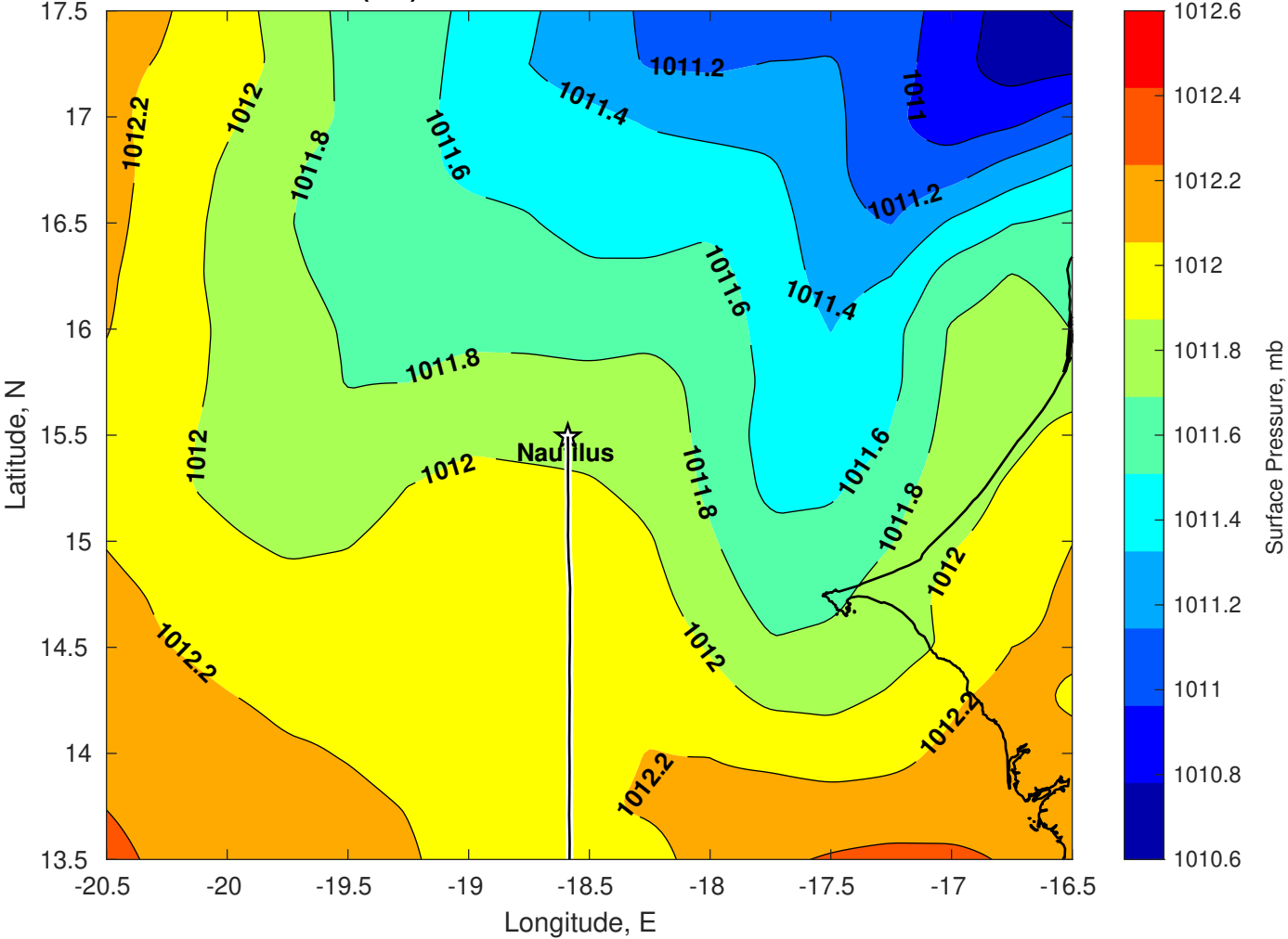
Surface Pressure (mb) for Nautilus at 12-Oct-2025 00:00:00
