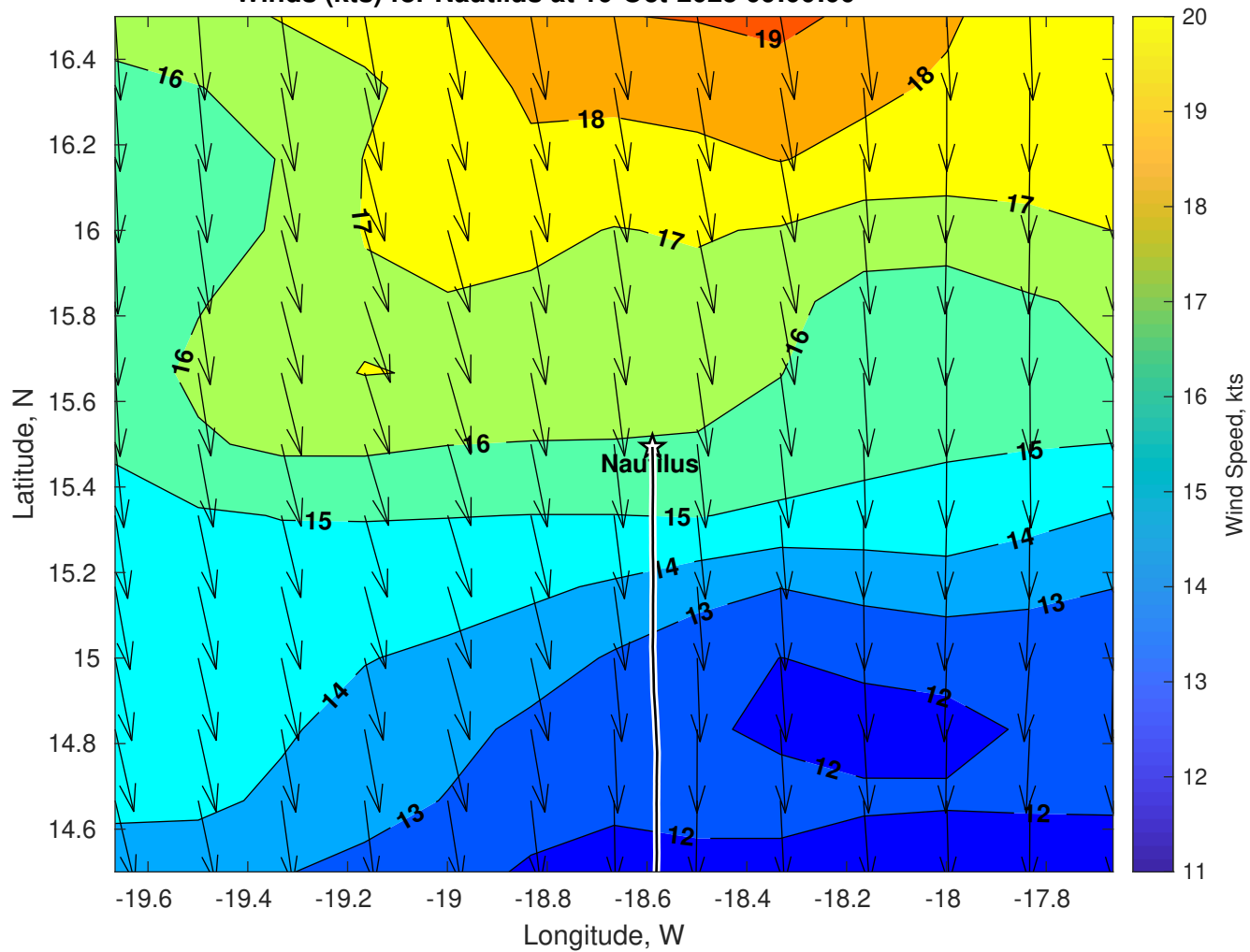
Winds (kts) for Nautilus at 10-Oct-2025 09:00:00
