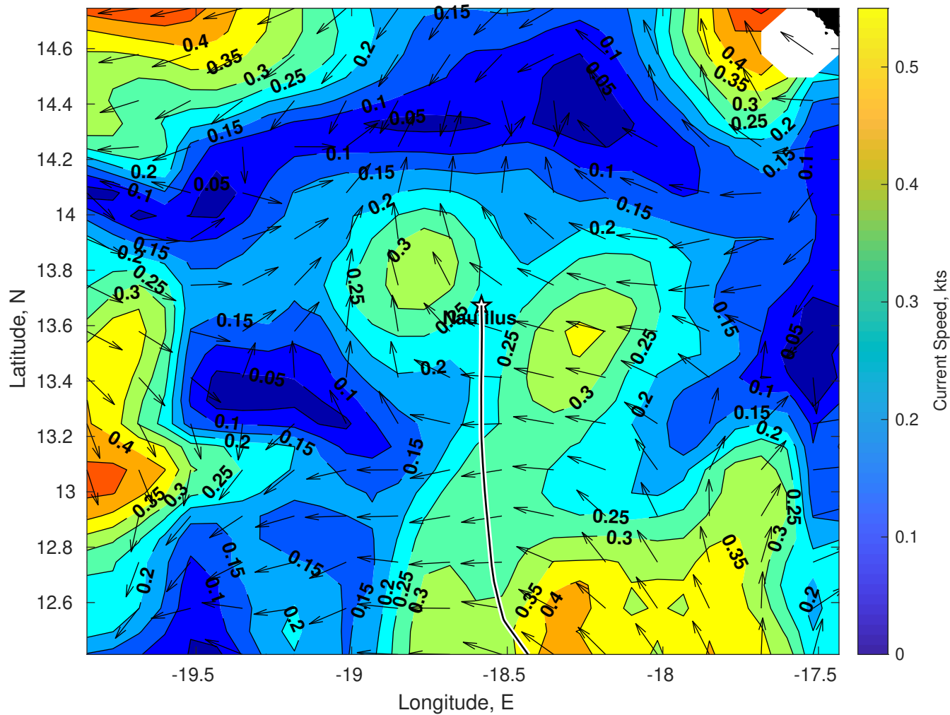
Surface Currents for Nautilus at 09-Oct-2025 00:00:00
