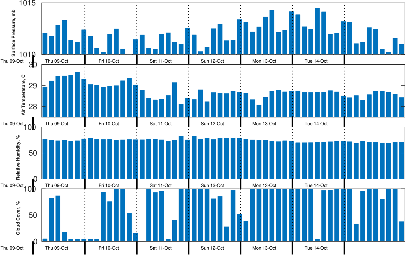
Met Forecast for Nautilus from 10-Oct-2025 00:00:00 to 17-Oct-2025 00:00:00
