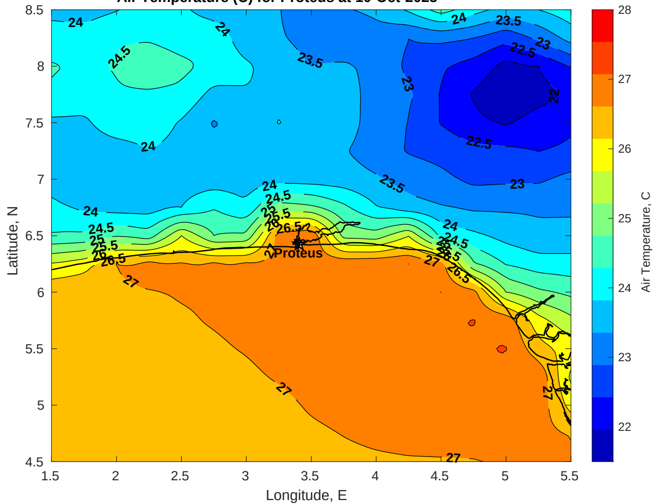
Air Temperature (C) for Proteus at 10-Oct-2025
