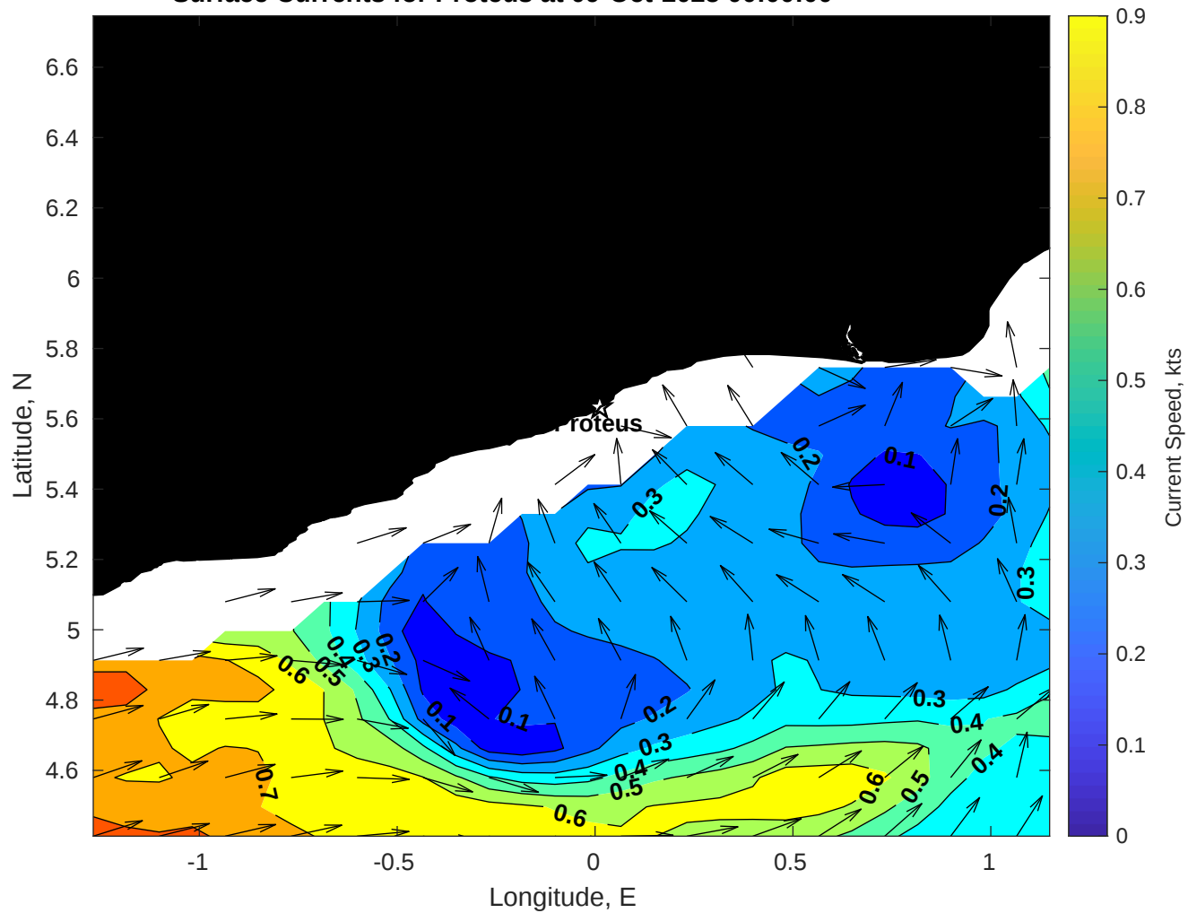
Surface Currents for Proteus at 09-Oct-2025 00:00:00
