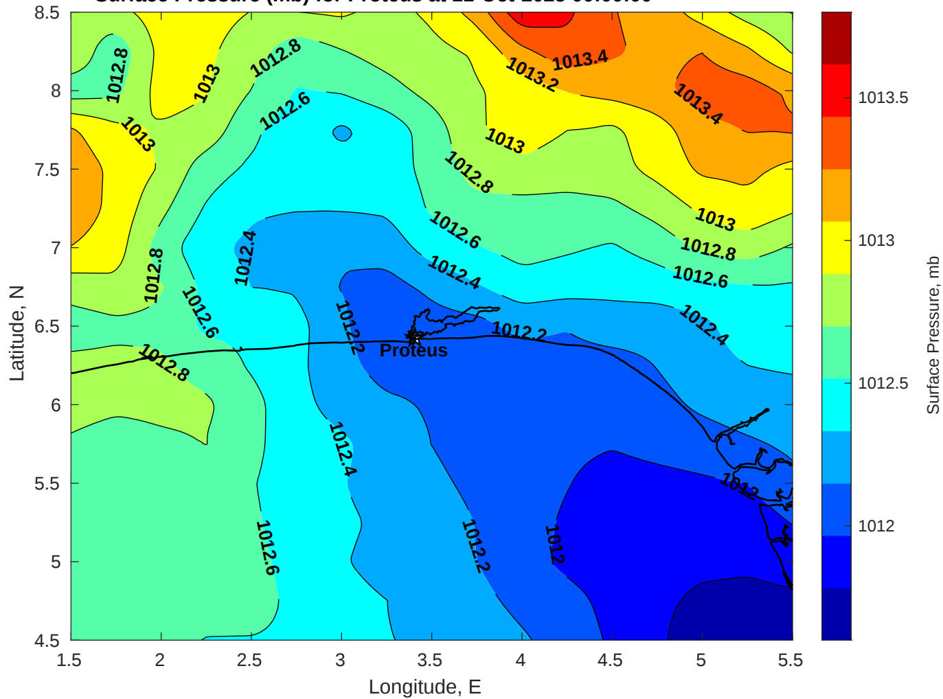
Surface Pressure (mb) for Proteus at 11-Oct-2025 00:00:00
