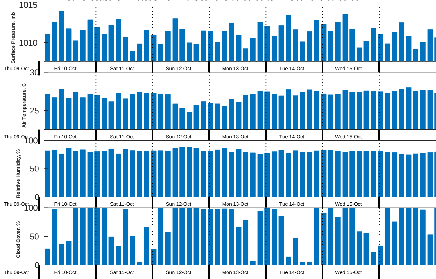
Met Forecast for Proteus from 10-Oct-2025 00:00:00 to 17-Oct-2025 00:00:00
