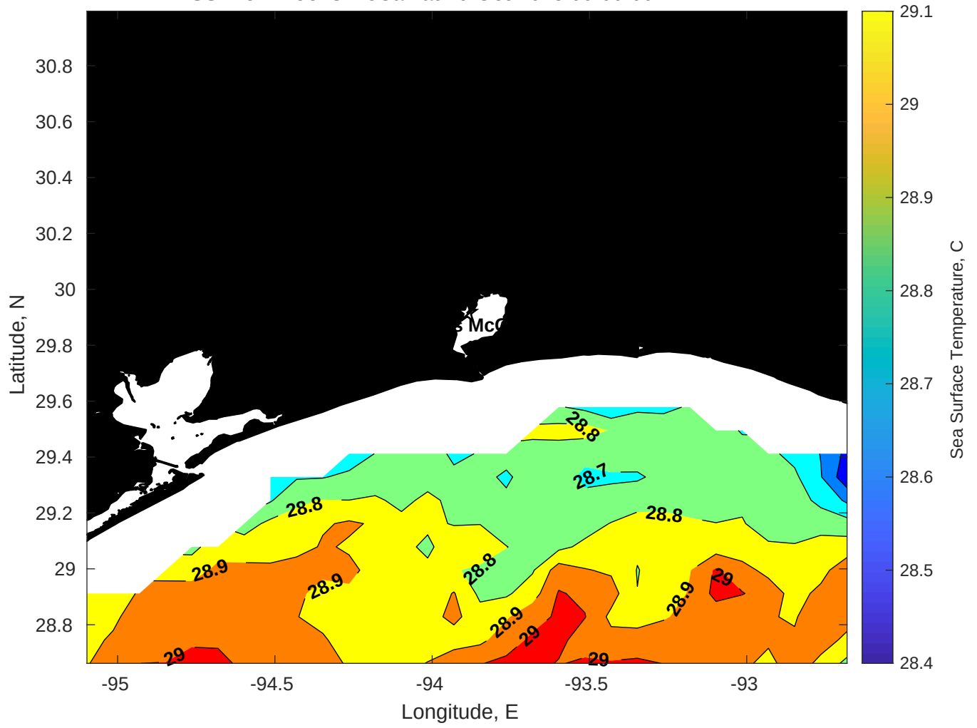
SST for Brooks McCall at 10-Oct-2025 00:00:00
