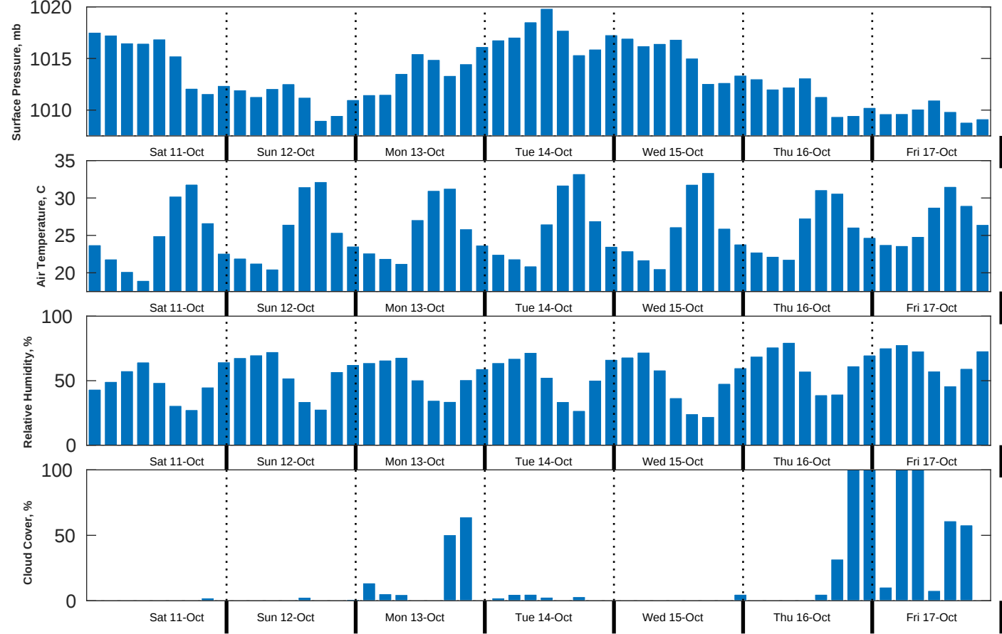
Met Forecast for Brooks McCall from 11-Oct-2025 00:00:00 to 18-Oct-2025 00:00:00
