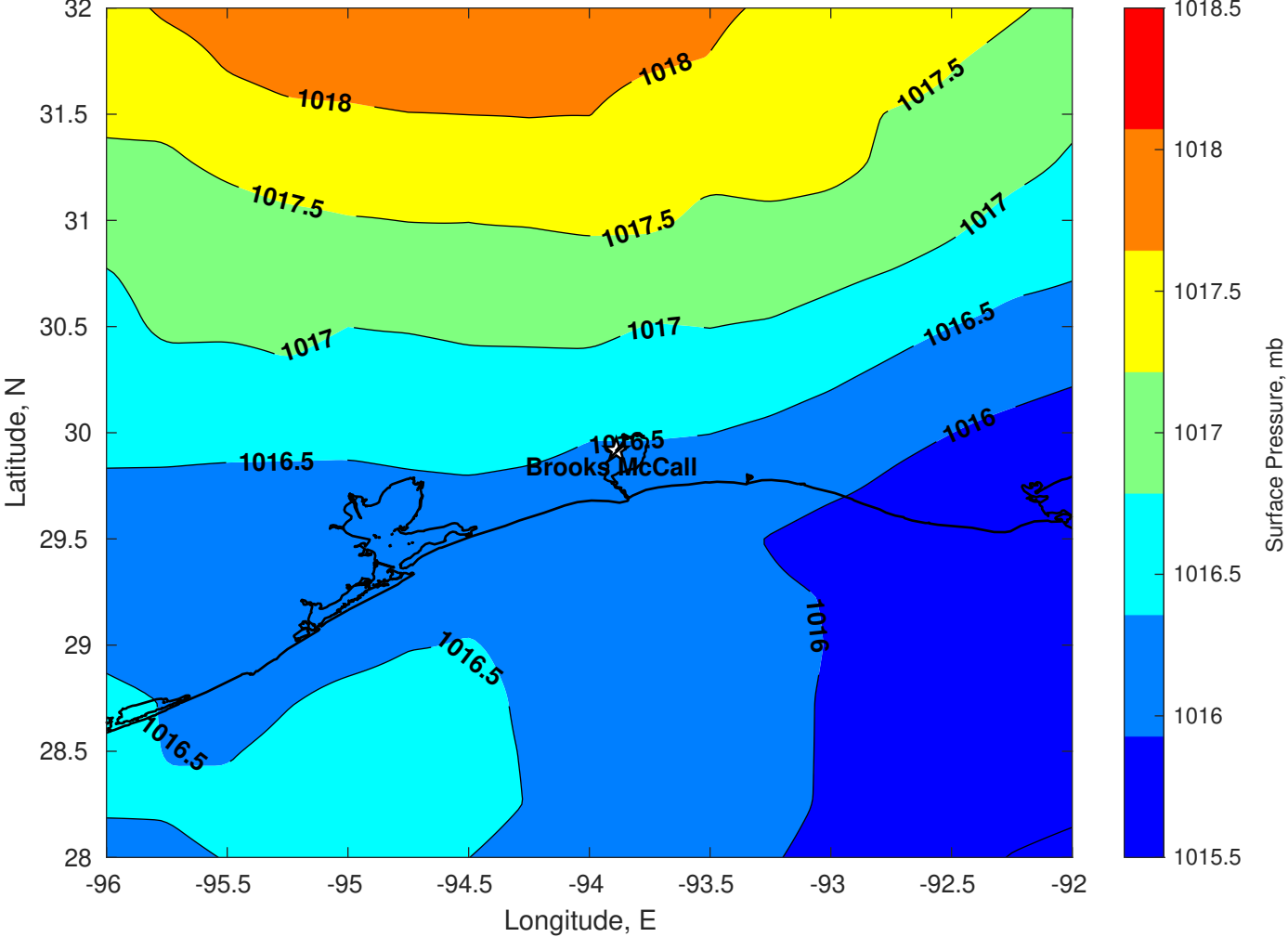
Surface Pressure (mb) for Brooks McCall at 11-Oct-2025 00:00:00
