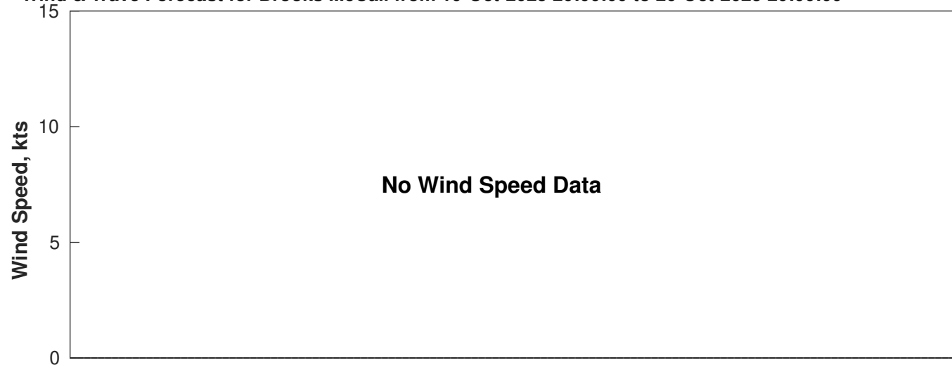
Wind & Wave Forecast for Brooks McCall from 10-Oct-2025 20:00:00 to 26-Oct-2025 20:00:00
