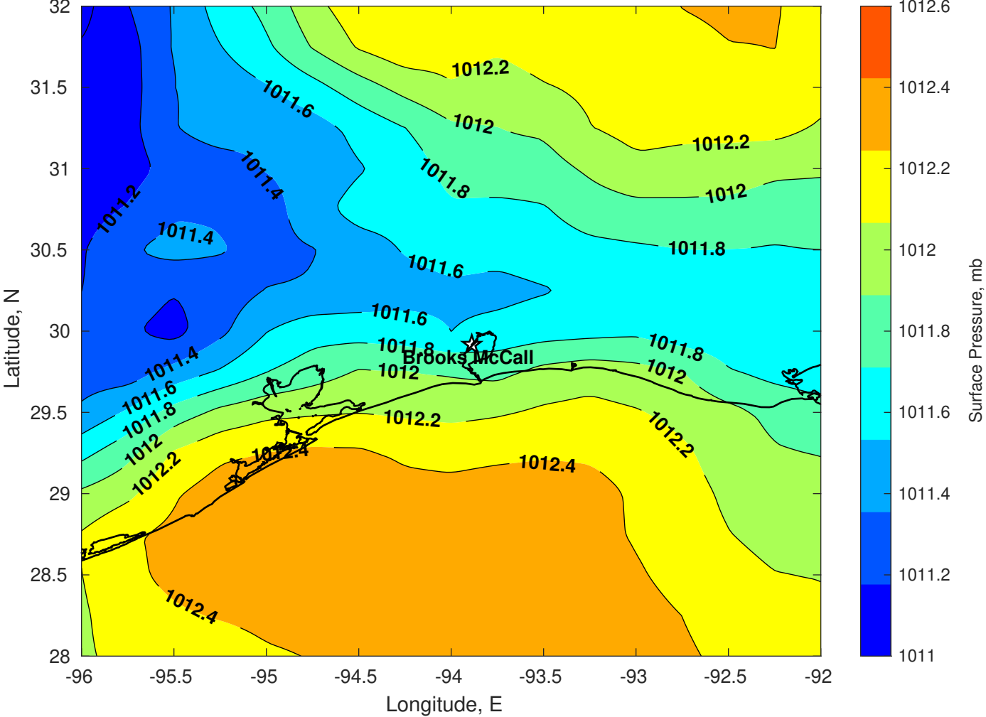
Surface Pressure (mb) for Brooks McCall at 12-Oct-2025 00:00:00
