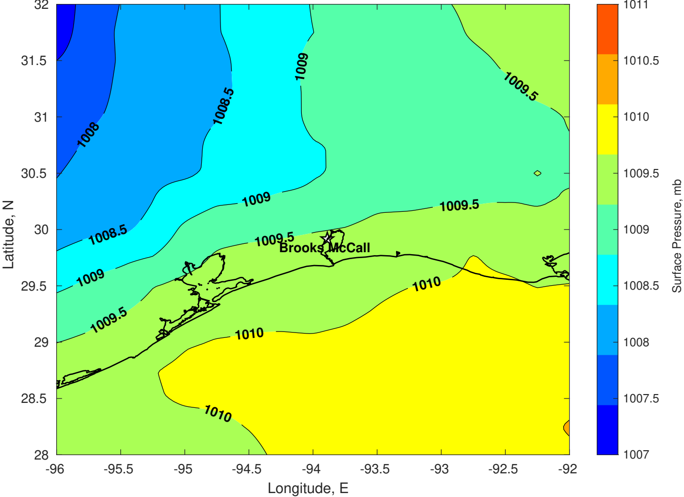
Surface Pressure (mb) for Brooks McCall at 13-Oct-2025 00:00:00
