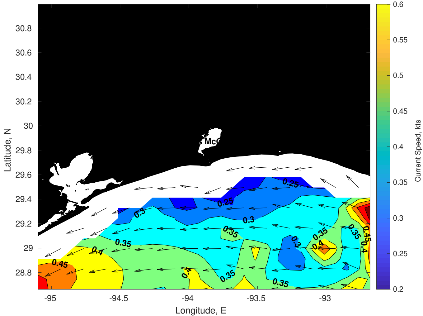
Surface Currents for Brooks McCall at 10-Oct-2025 00:00:00
