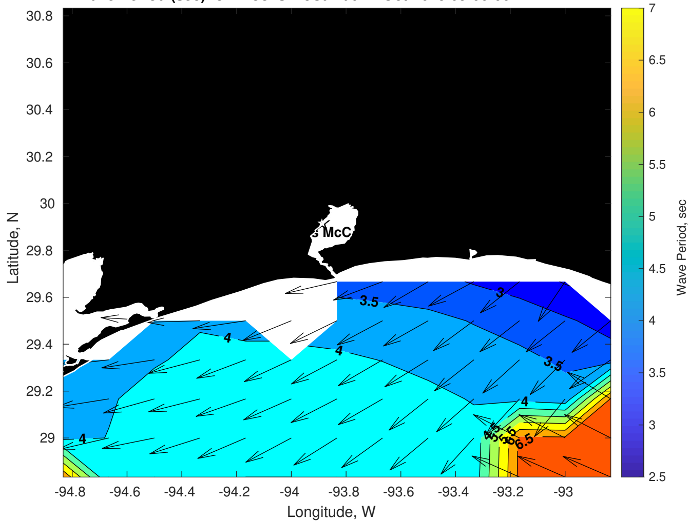
Wave Period (sec) for Brooks McCall at 11-Oct-2025 09:00:00
