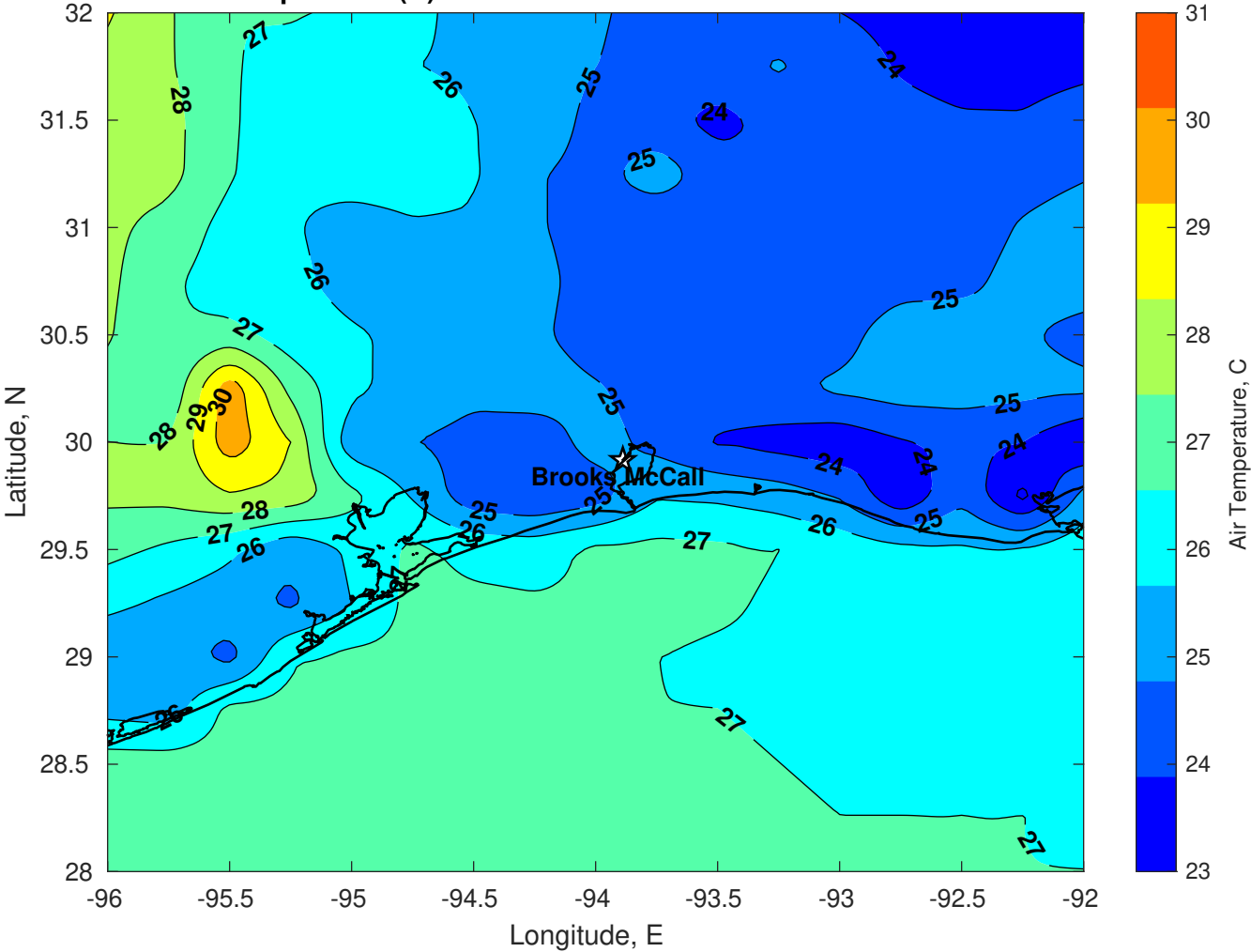
Air Temperature (C) for Brooks McCall at 11-Oct-2025
