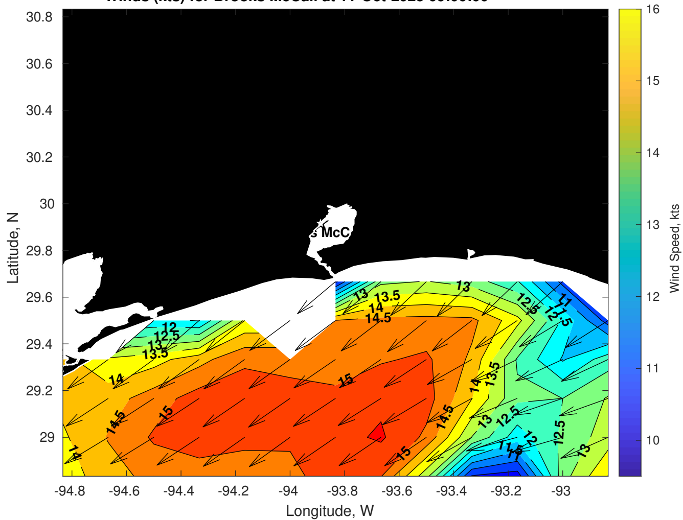
Winds (kts) for Brooks McCall at 11-Oct-2025 09:00:00
