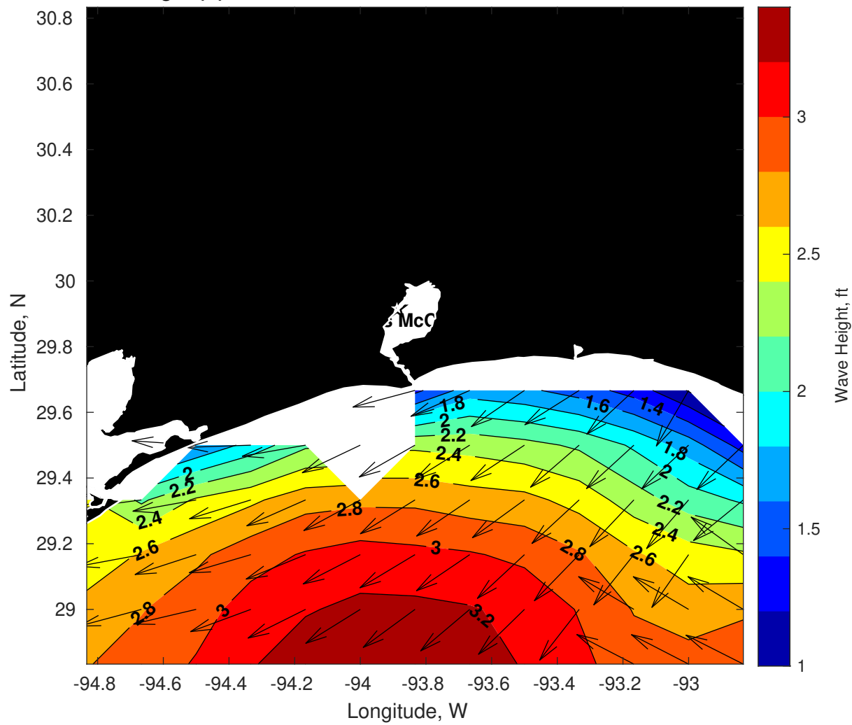
Wave Height (ft) for Brooks McCall at 11-Oct-2025 09:00:00
