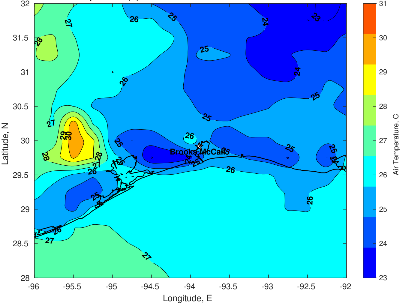
Air Temperature (C) for Brooks McCall at 11-Oct-2025
