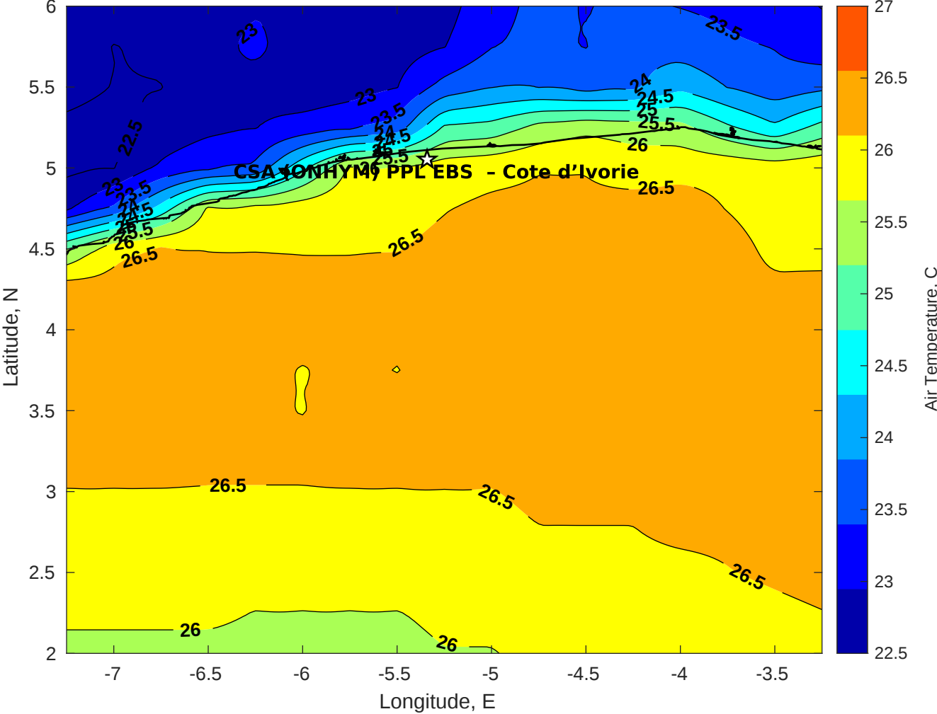
Air Temperature (C) for CSA (ONHYM) PPL EBS - Cote d'Ivoire at 11-Oct-2025
