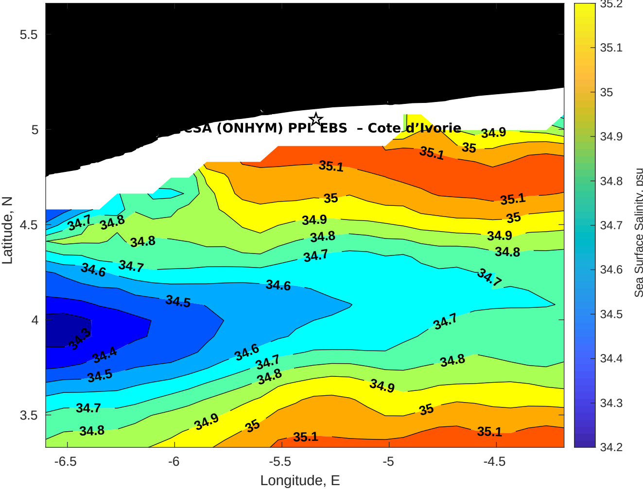
Surface Salinity for CSA (ONHYM) PPL EBS - Cote d'Ivoire at 10-Oct-2025 00:00:00
