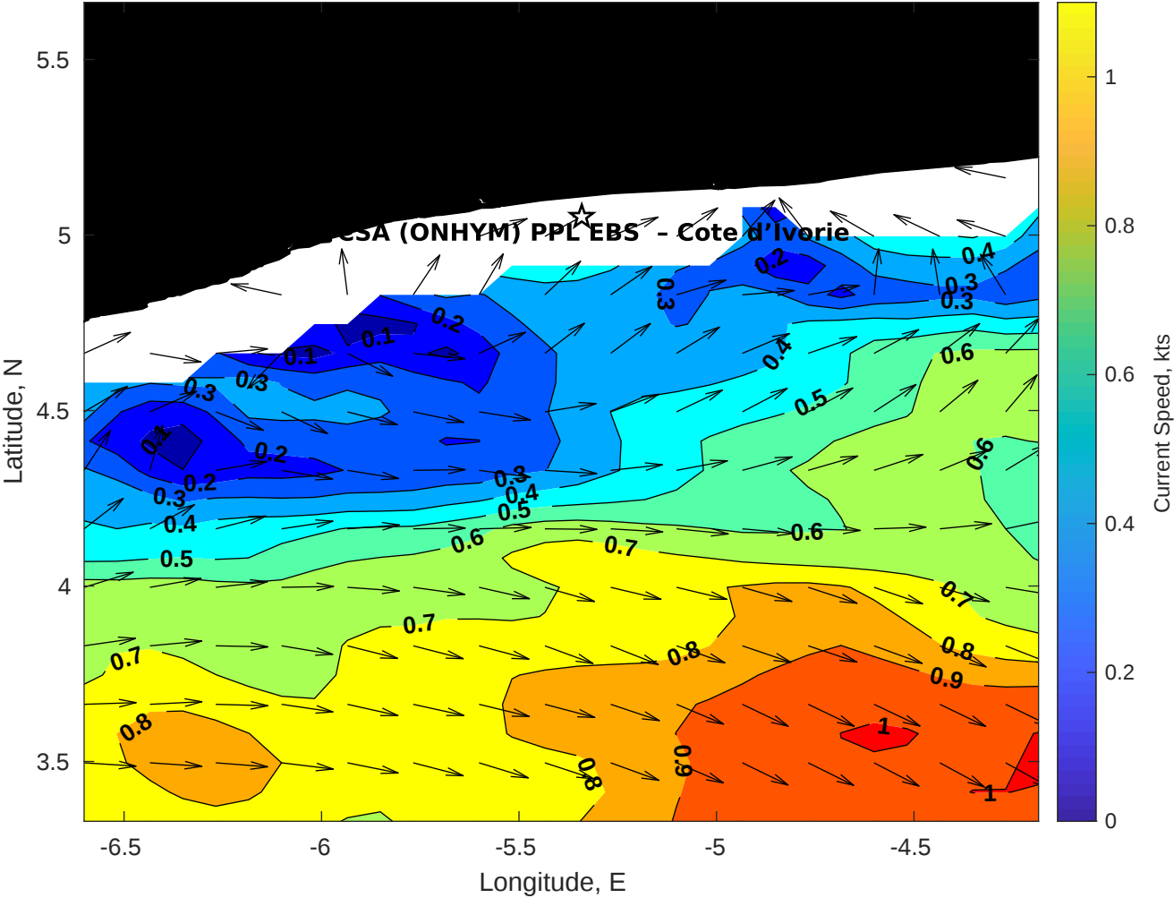
Surface Currents for CSA (ONHYM) PPL EBS - Cote d'Ivoire at 10-Oct-2025 00:00:00
