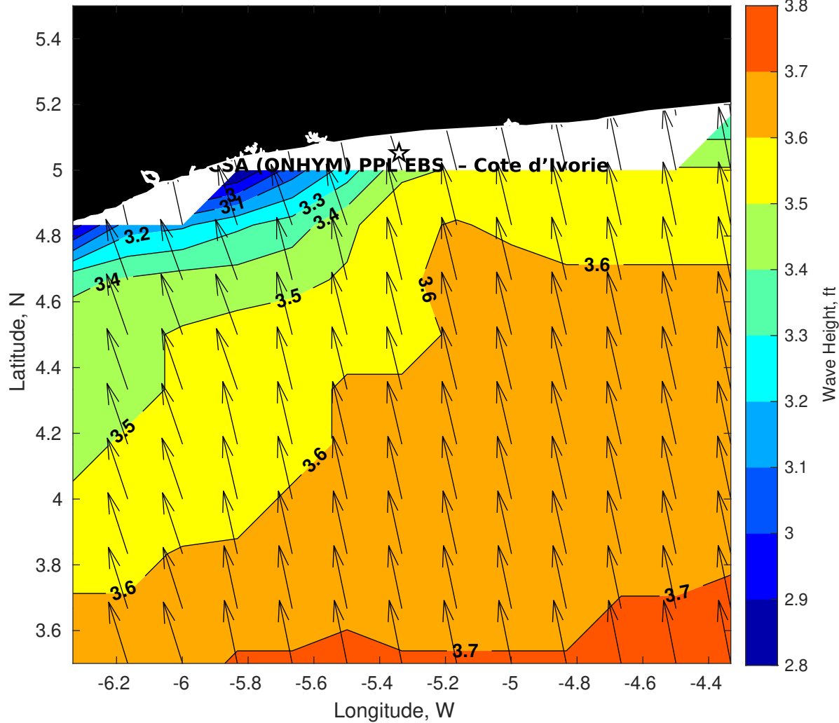
Wave Height (ft) for CSA (ONHYM) PPL EBS - Cote d'Ivoire at 11-Oct-2025 09:00:00
