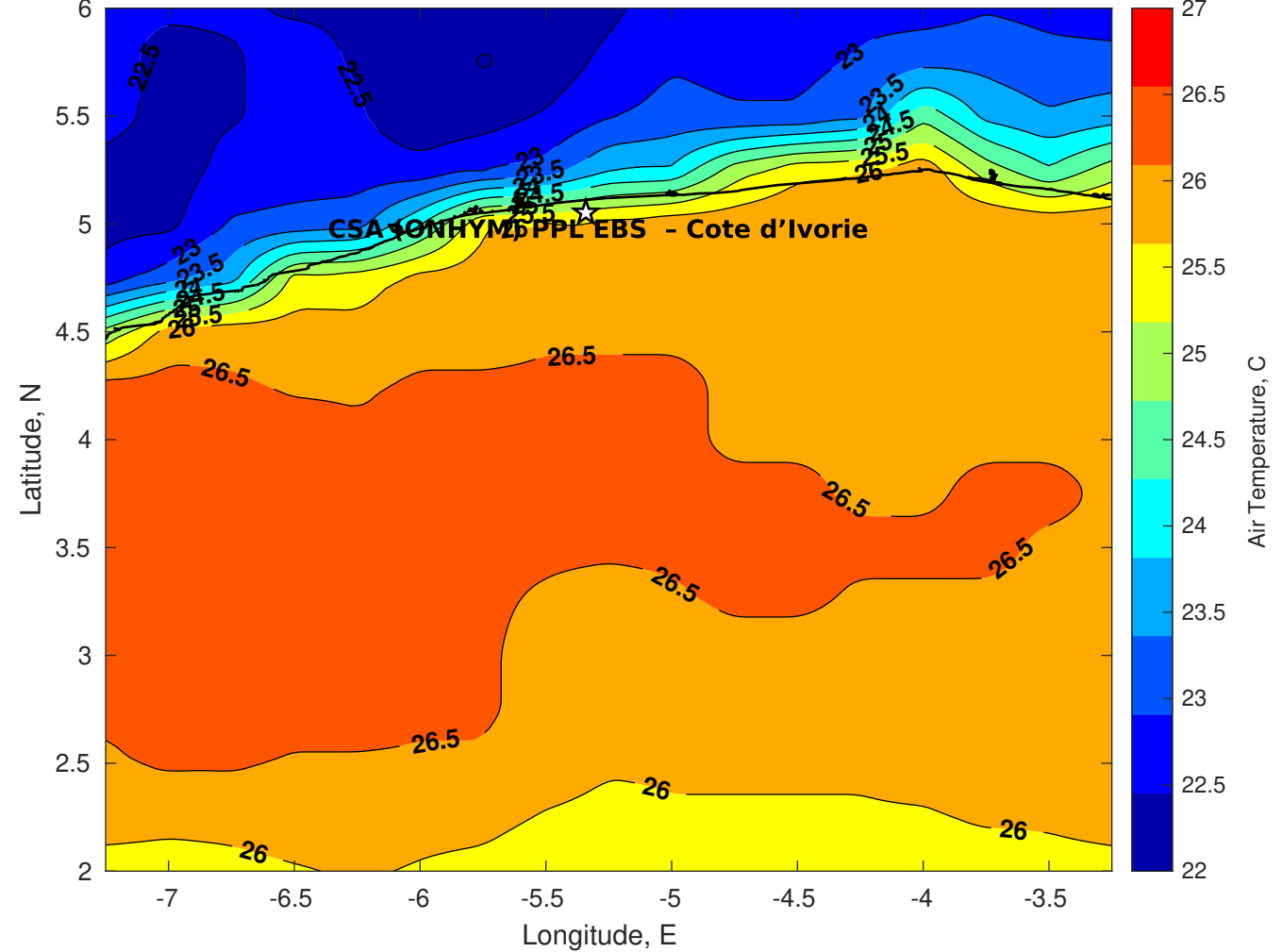
Air Temperature (C) for CSA (ONHYM) PPL EBS - Cote d'Ivoire at 11-Oct-2025
