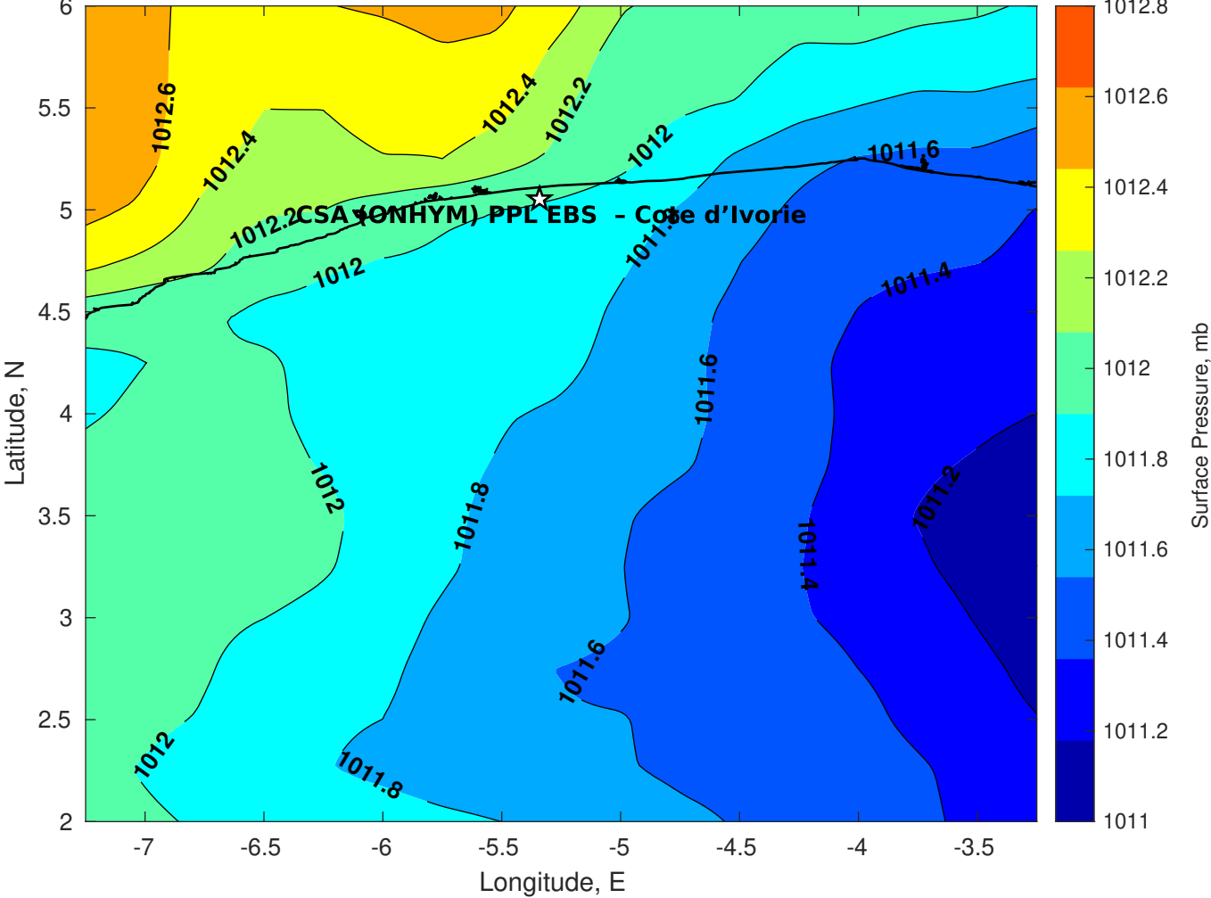
Surface Pressure (mb) for CSA (ONHYM) PPL EBS - Cote d'Ivoire at 13-Oct-2025 00:00:00
