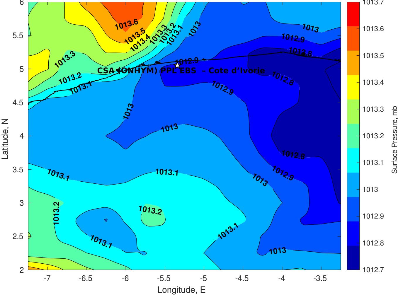
Surface Pressure (mb) for CSA (ONHYM) PPL EBS - Cote d'Ivoire at 11-Oct-2025 00:00:00
