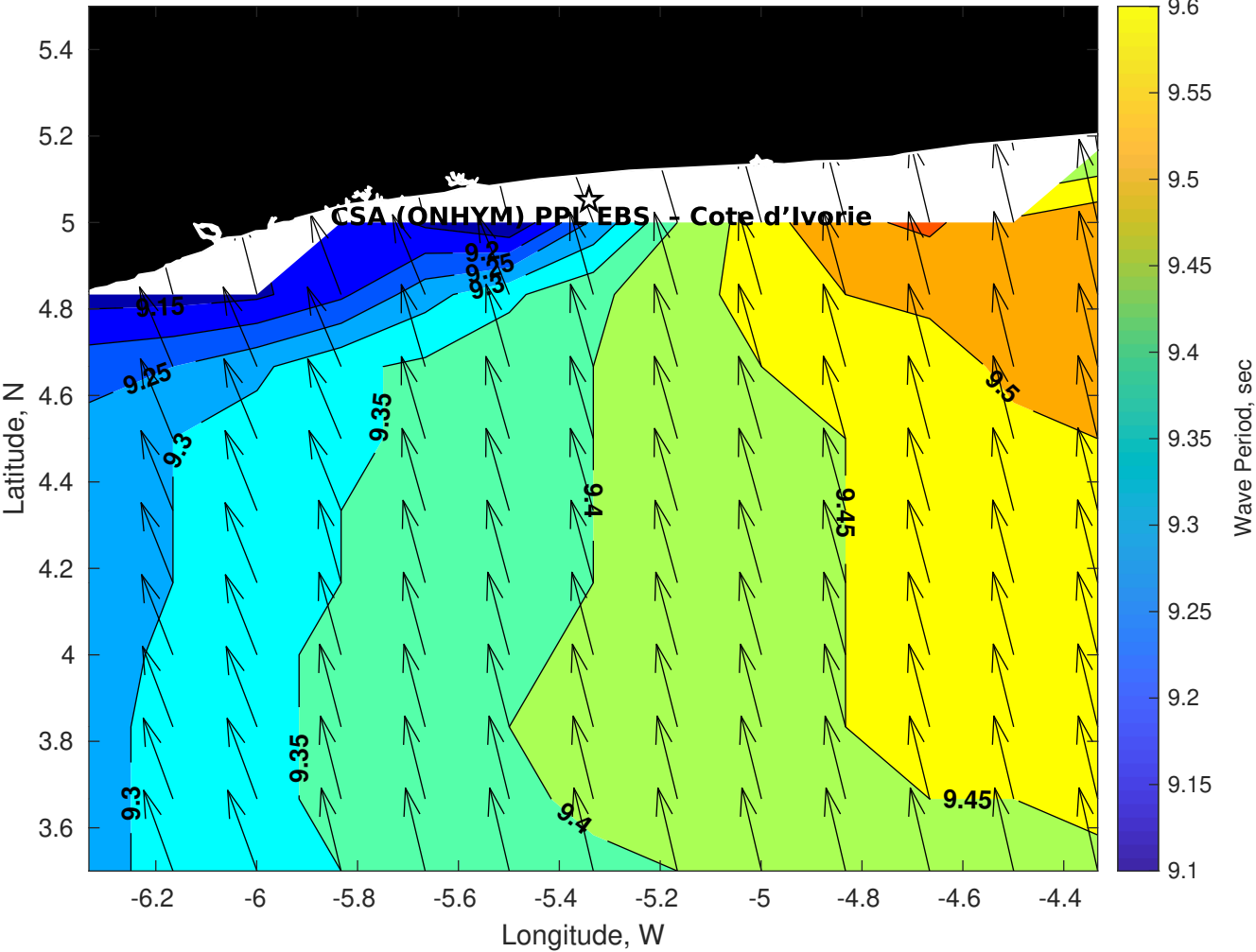
Wave Period (sec) for CSA (ONHYM) PPL EBS - Cote d'Ivoire at 11-Oct-2025 09:00:00
