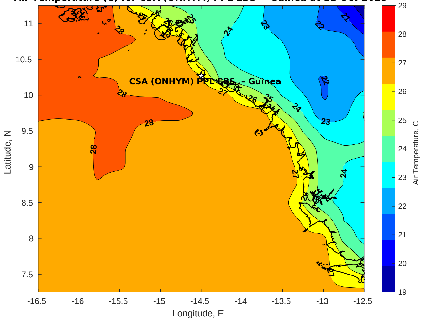
Air Temperature (C) for CSA (ONHYM) PPL EBS - Guinea at 11-Oct-2025
