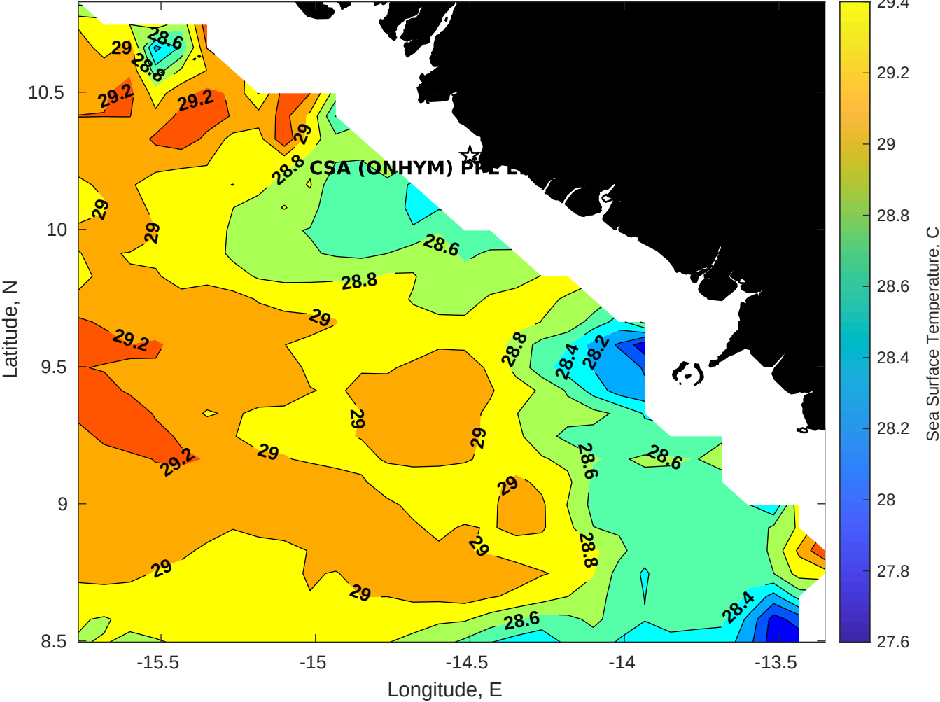
SST for CSA (ONHYM) PPL EBS - Guinea at 10-Oct-2025 00:00:00
