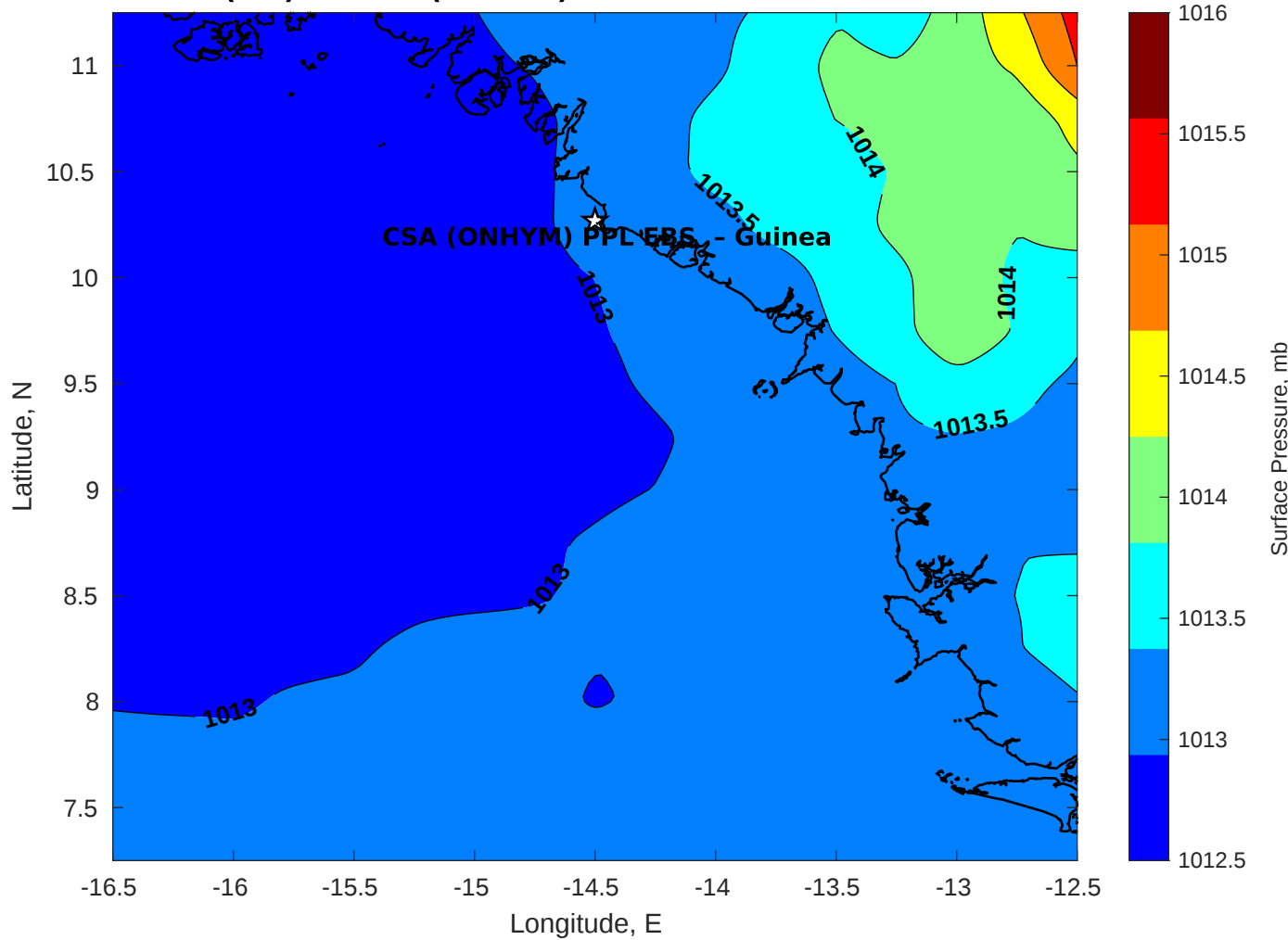
Surface Pressure (mb) for CSA (ONHYM) PPL EBS - Guinea at 11-Oct-2025 00:00:00
