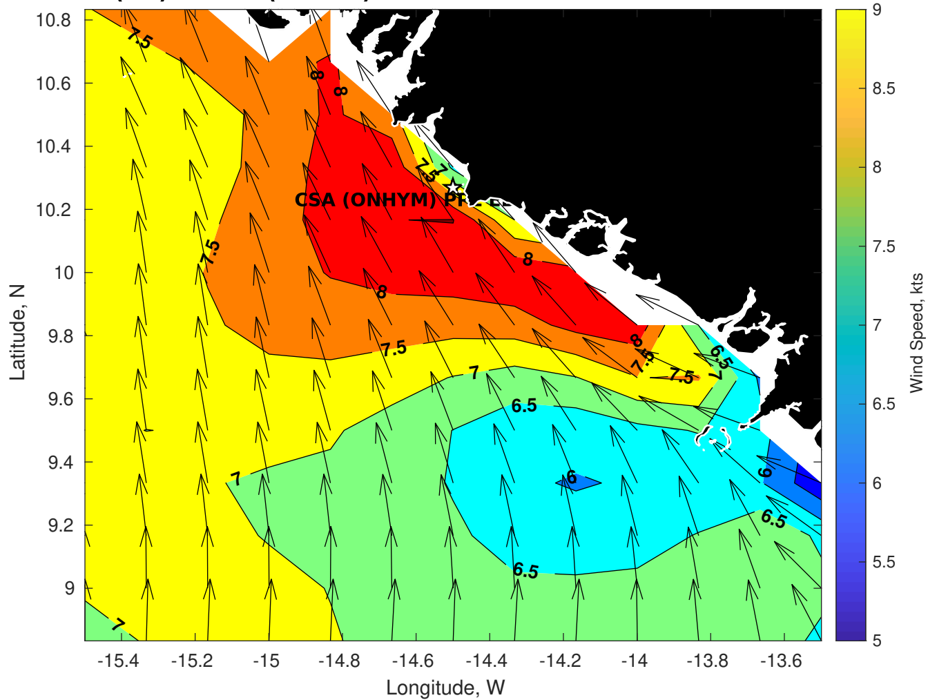
Winds (kts) for CSA (ONHYM) PPL EBS - Guinea at 11-Oct-2025 09:00:00
