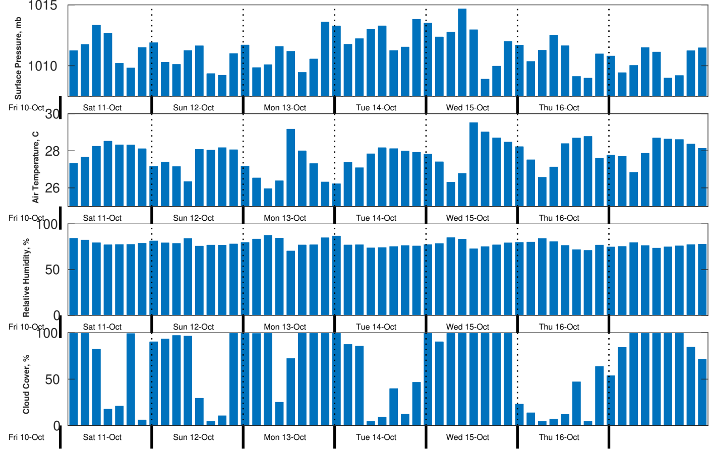
Met Forecast for CSA (ONHYM) PPL EBS - Guinea from 11-Oct-2025 00:00:00 to 18-Oct-2025 00:00:00
