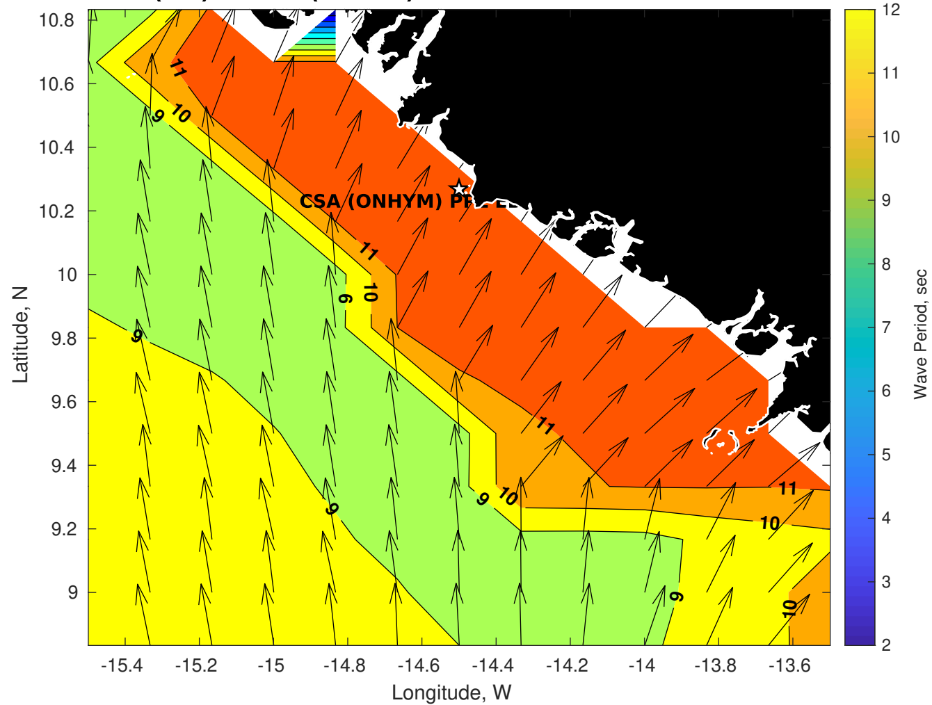
Wave Period (sec) for CSA (ONHYM) PPL EBS - Guinea at 11-Oct-2025 09:00:00
