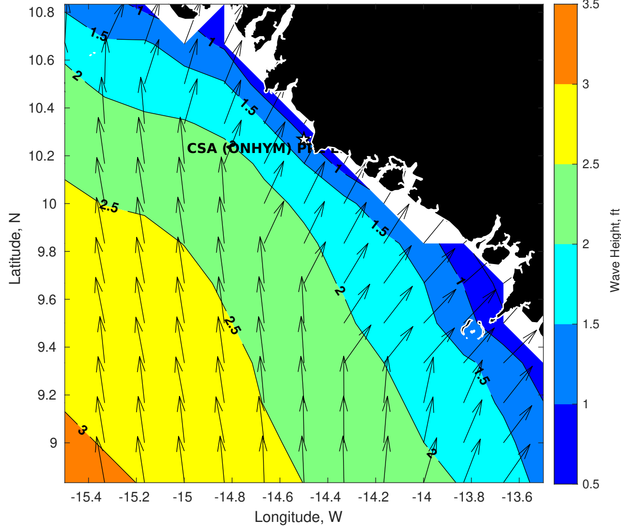
Wave Height (ft) for CSA (ONHYM) PPL EBS - Guinea at 11-Oct-2025 09:00:00
