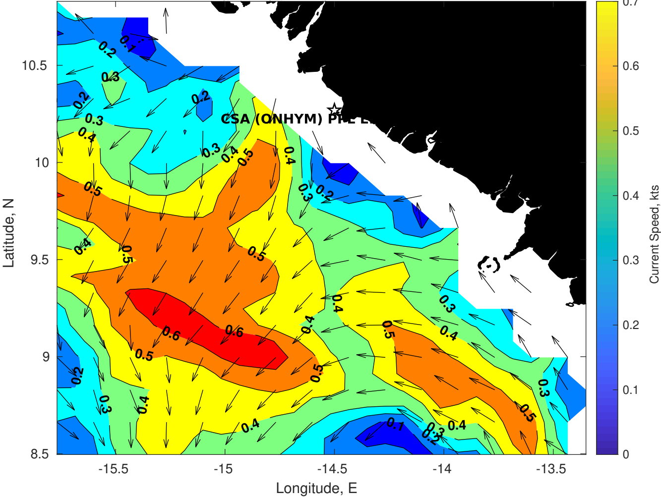
Surface Currents for CSA (ONHYM) PPL EBS - Guinea at 10-Oct-2025 00:00:00
