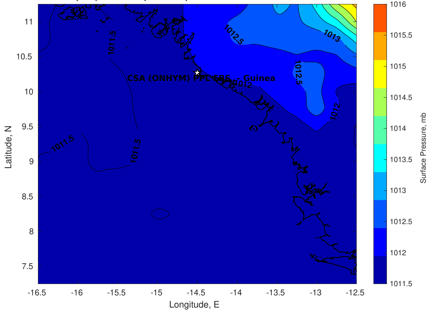
Surface Pressure (mb) for CSA (ONHYM) PPL EBS - Guinea at 12-Oct-2025 00:00:00
