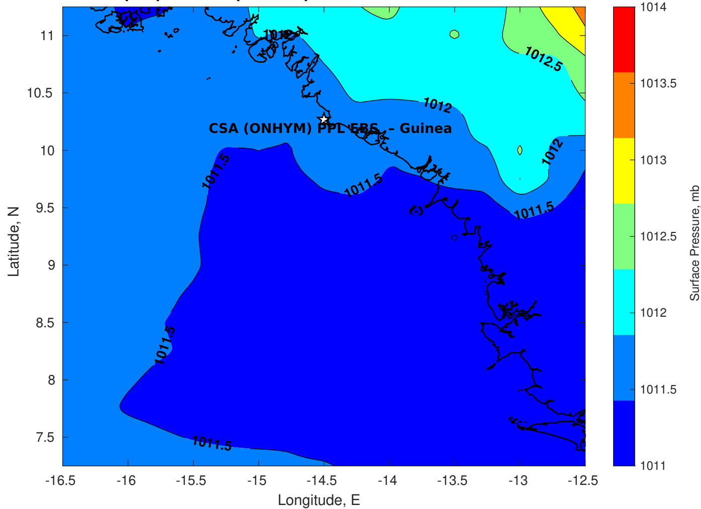
Surface Pressure (mb) for CSA (ONHYM) PPL EBS - Guinea at 13-Oct-2025 00:00:00
