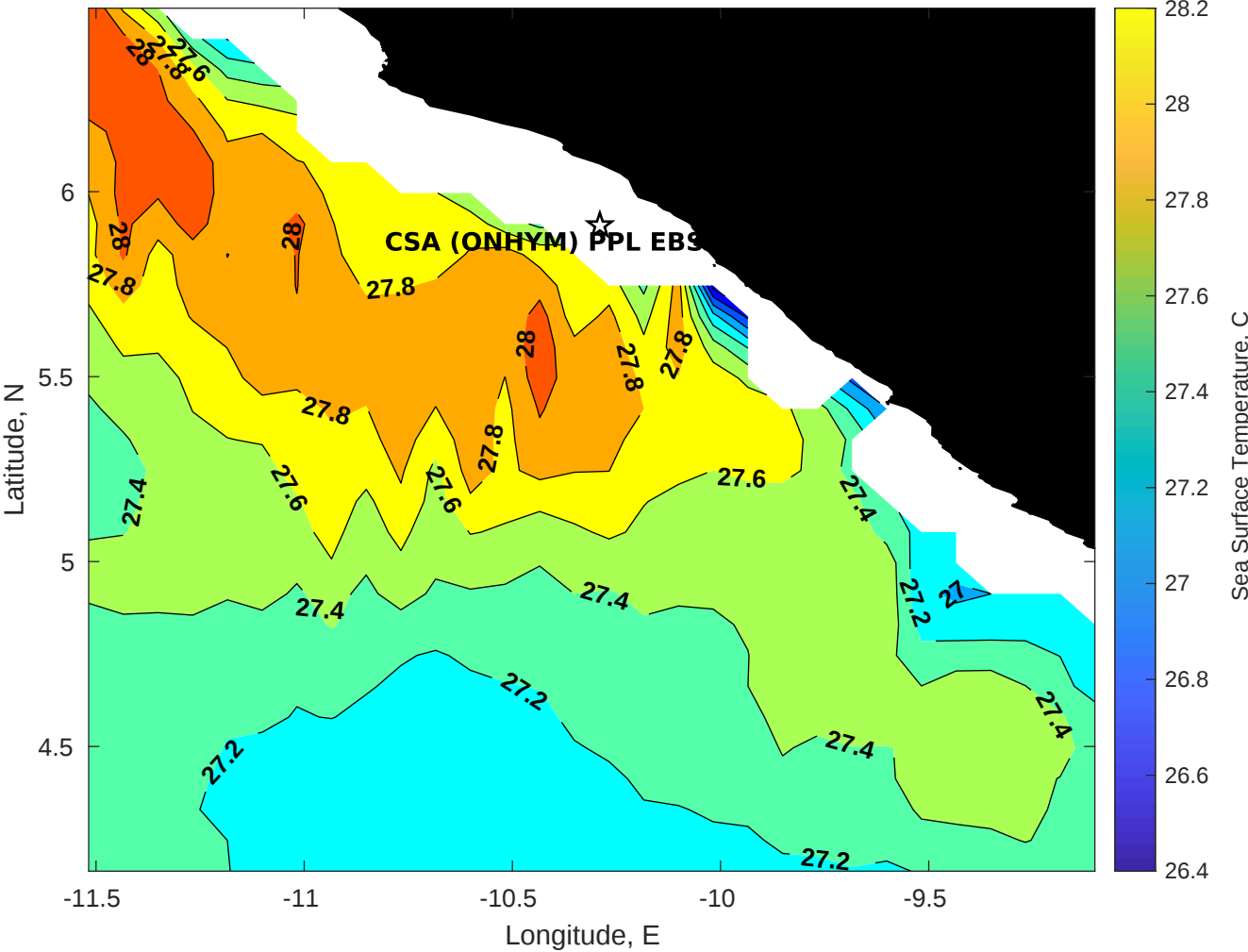
SST for CSA (ONHYM) PPL EBS - Liberia at 10-Oct-2025 00:00:00
