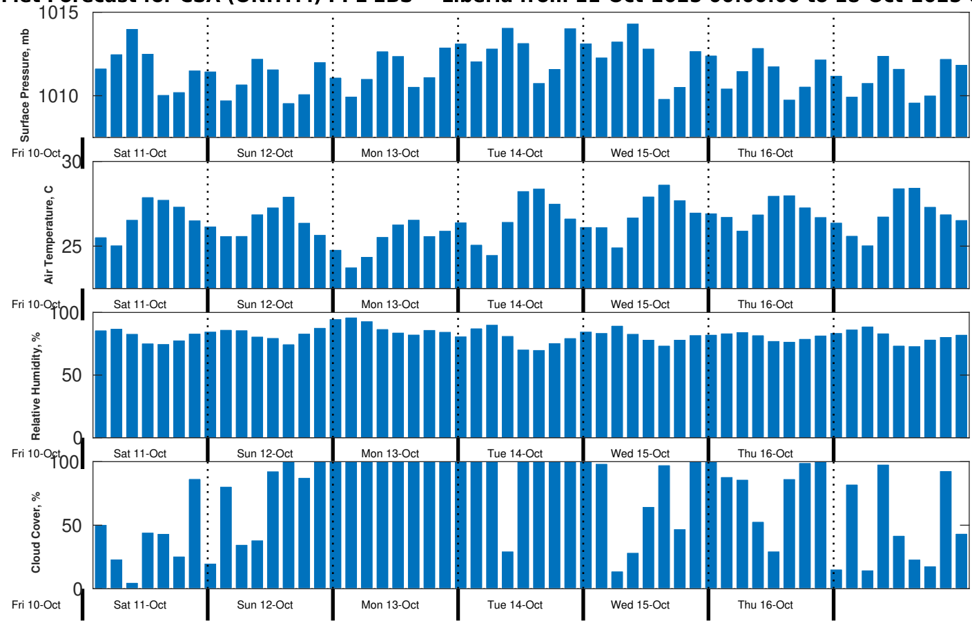
Met Forecast for CSA (ONHYM) PPL EBS - Liberia from 11-Oct-2025 00:00:00 to 18-Oct-2025 00:00:00
