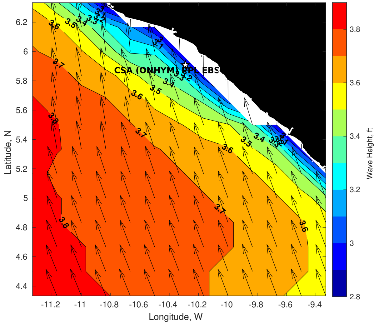
Wave Height (ft) for CSA (ONHYM) PPL EBS - Liberia at 11-Oct-2025 09:00:00
