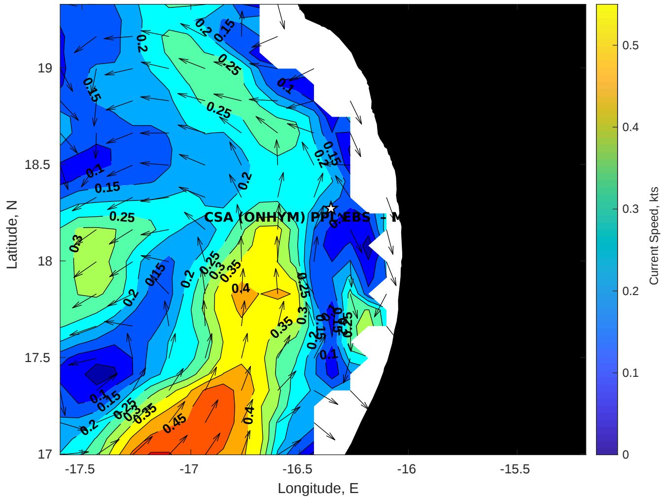
Surface Currents for CSA (ONHYM) PPL EBS - Mauritania at 10-Oct-2025 00:00:00
