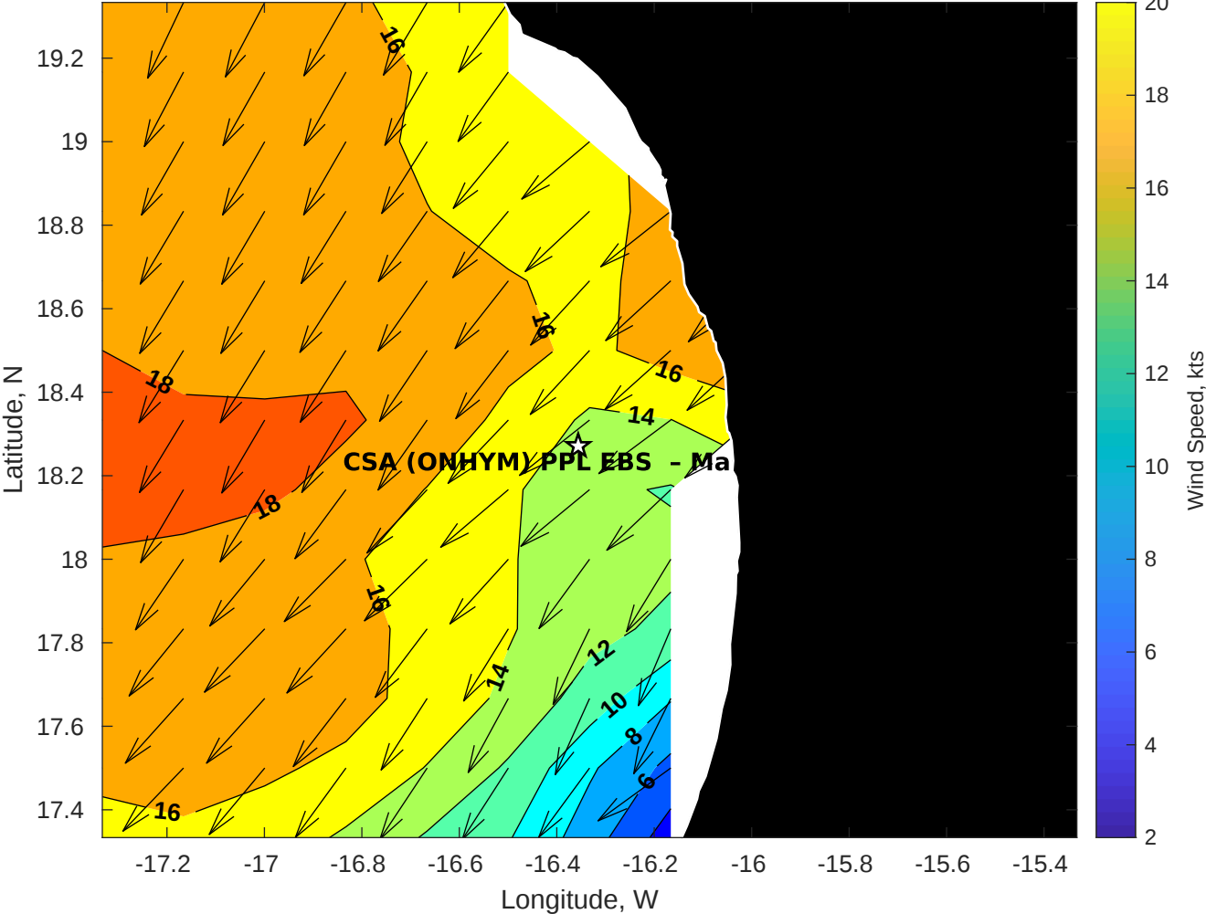
Winds (kts) for CSA (ONHYM) PPL EBS - Mauritania at 11-Oct-2025 09:00:00
