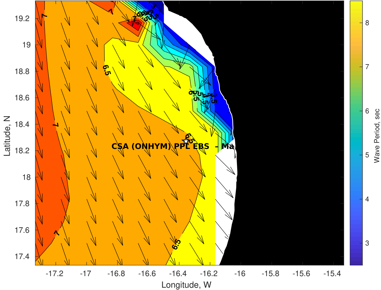
Wave Period (sec) for CSA (ONHYM) PPL EBS - Mauritania at 11-Oct-2025 09:00:00
