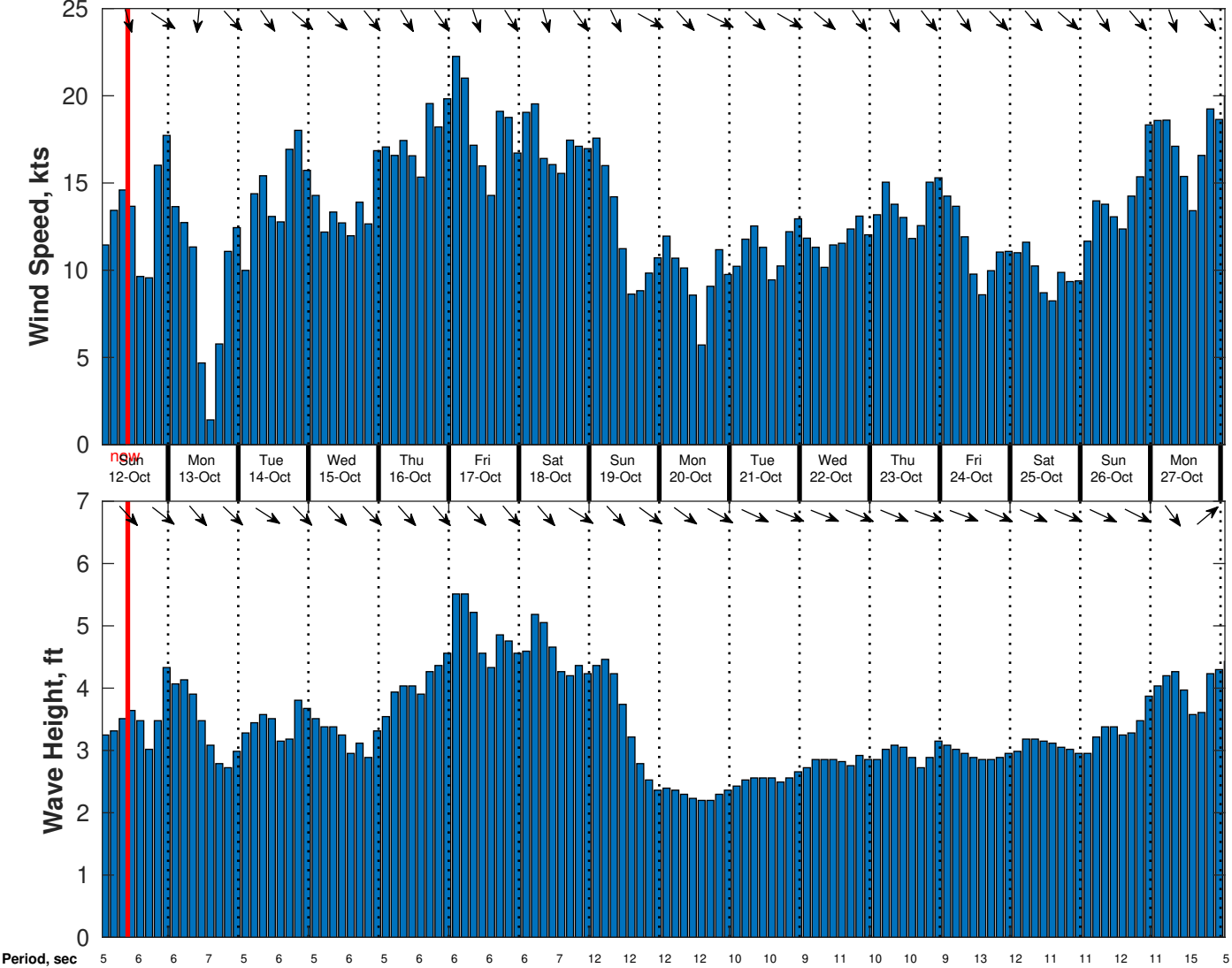
Wind & Wave Forecast for CSA (ONHYM) PPL EBS - Mauritania from 11-Oct-2025 01:00:00 to 27-Oct-2025 01:00:00
