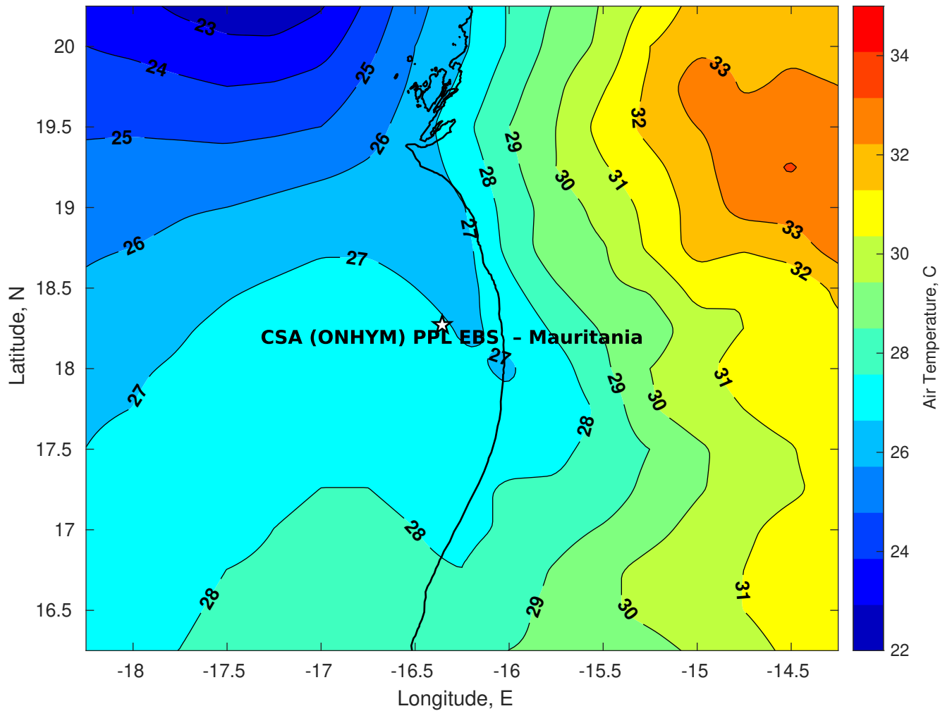
Air Temperature (C) for CSA (ONHYM) PPL EBS - Mauritania at 11-Oct-2025
