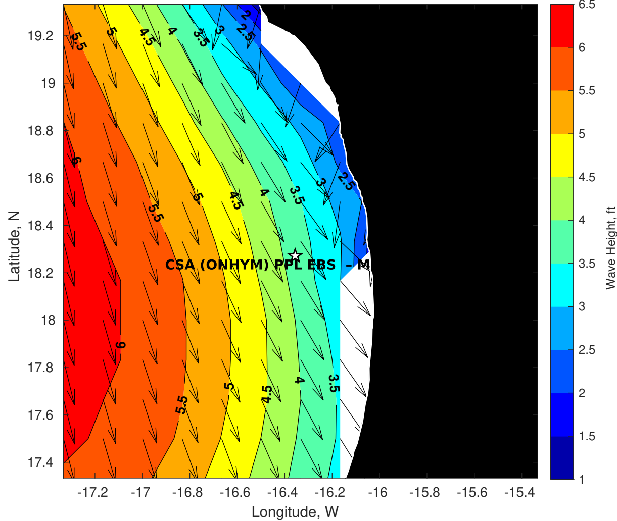
Wave Height (ft) for CSA (ONHYM) PPL EBS - Mauritania at 11-Oct-2025 09:00:00
