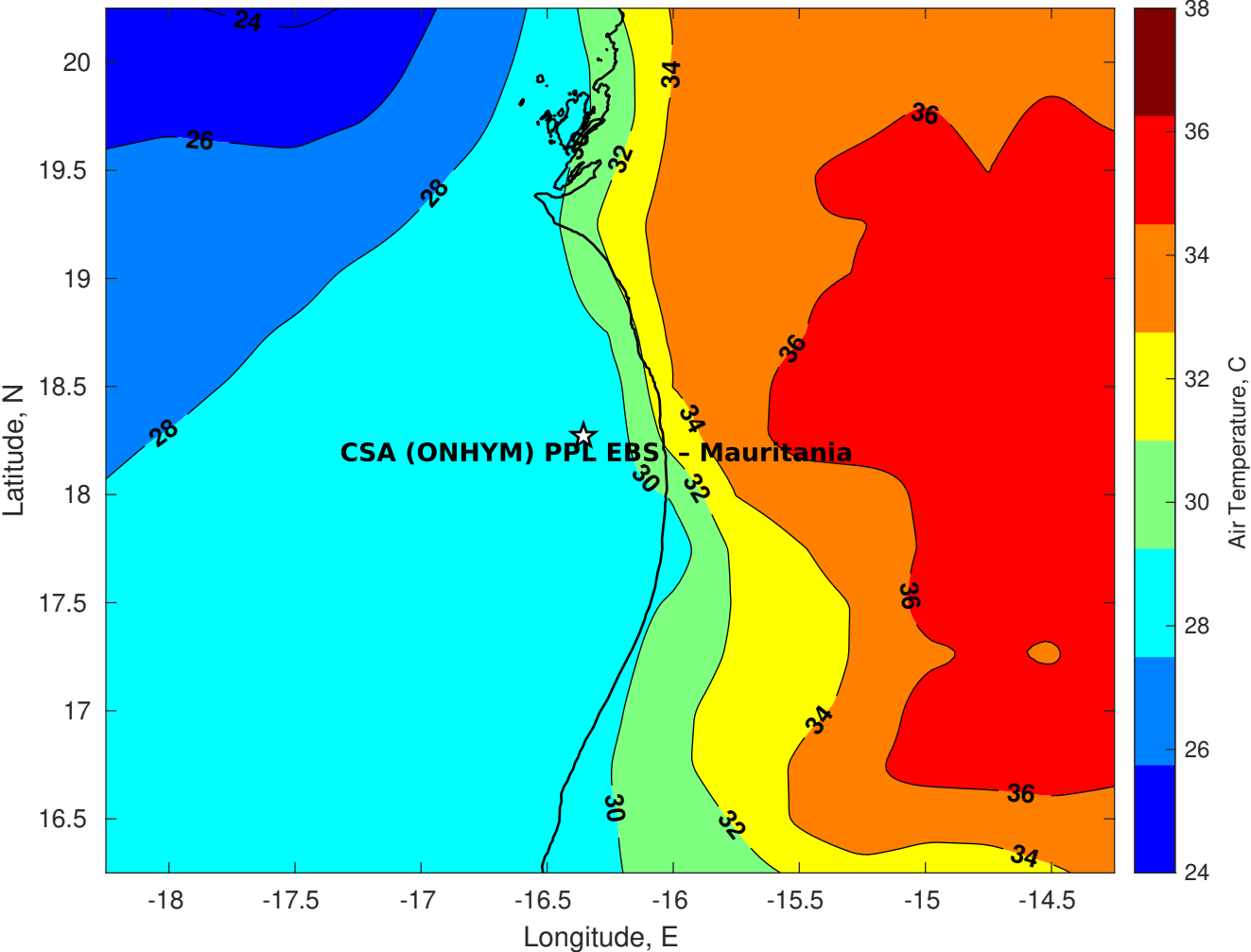
Air Temperature (C) for CSA (ONHYM) PPL EBS - Mauritania at 11-Oct-2025
