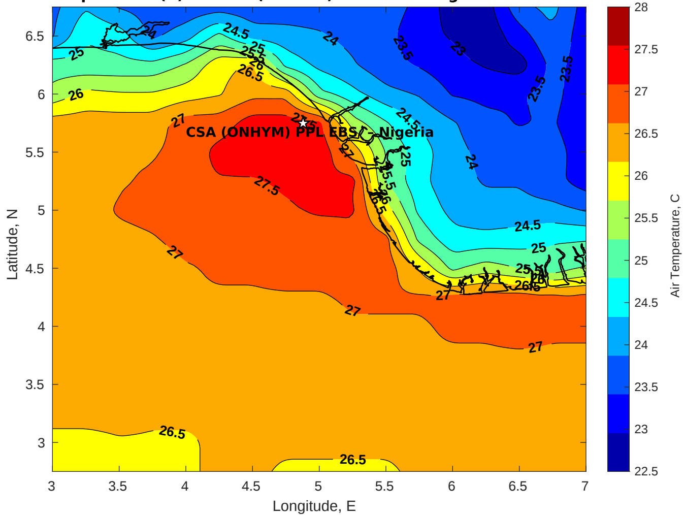
Air Temperature (C) for CSA (ONHYM) PPL EBS - Nigeria at 11-Oct-2025
