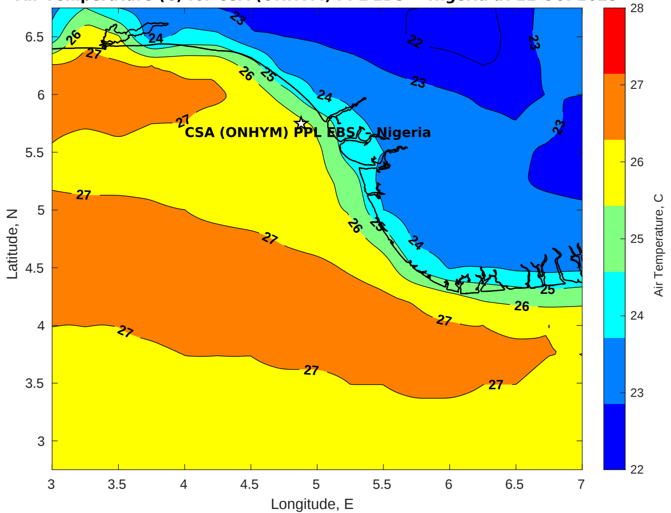
Air Temperature (C) for CSA (ONHYM) PPL EBS - Nigeria at 11-Oct-2025
