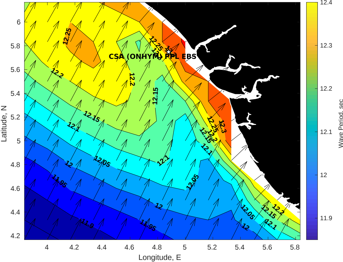
Wave Period (sec) for CSA (ONHYM) PPL EBS - Nigeria at 11-Oct-2025 09:00:00
