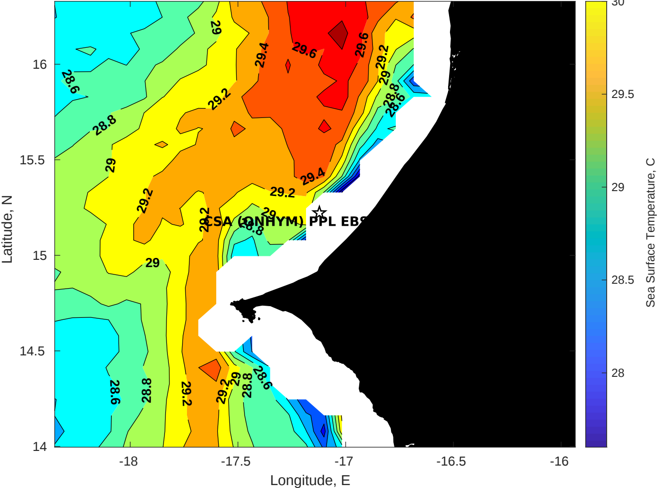
SST for CSA (ONHYM) PPL EBS - Senegal at 10-Oct-2025 00:00:00
