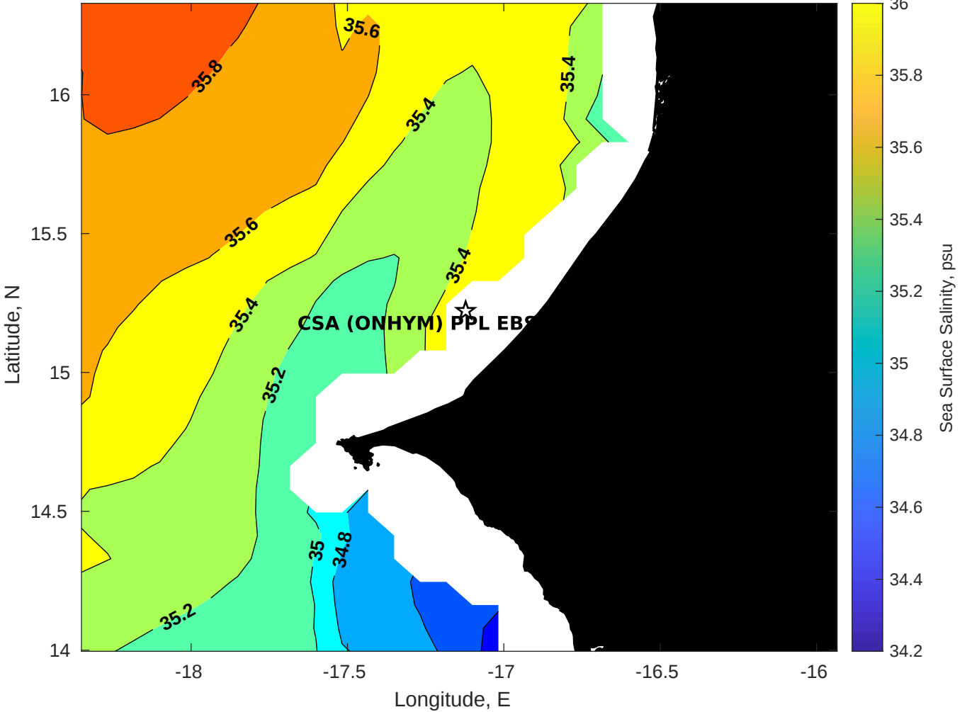
Surface Salinity for CSA (ONHYM) PPL EBS - Senegal at 10-Oct-2025 00:00:00
