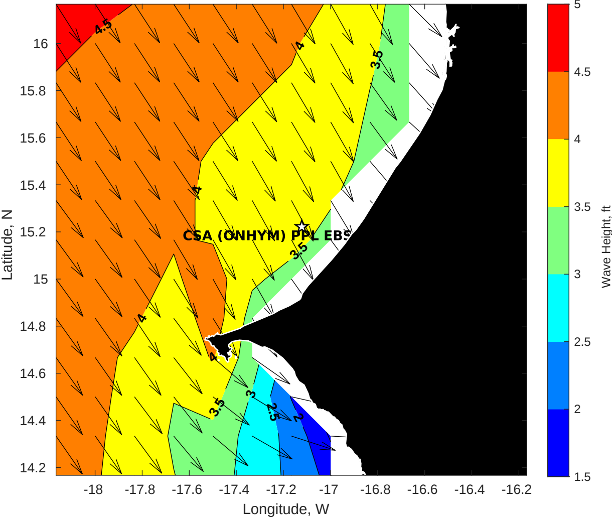
Wave Height (ft) for CSA (ONHYM) PPL EBS - Senegal at 11-Oct-2025 09:00:00
