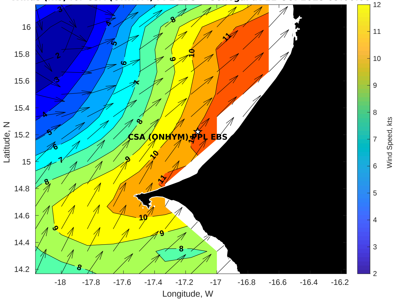
Winds (kts) for CSA (ONHYM) PPL EBS - Senegal at 11-Oct-2025 09:00:00
