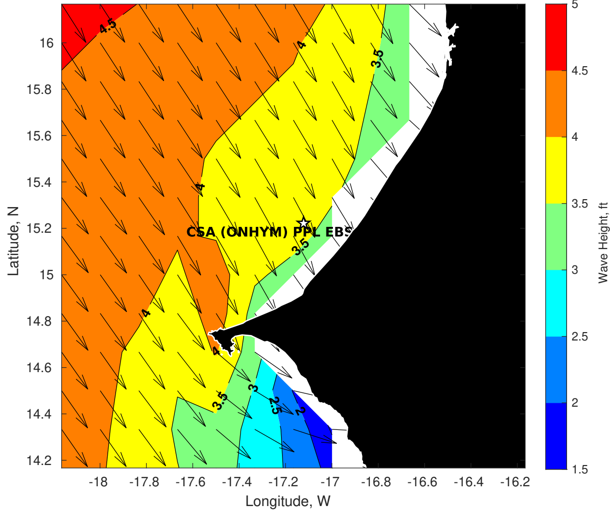
Wave Height (ft) for CSA (ONHYM) PPL EBS - Senegal at 11-Oct-2025 09:00:00
