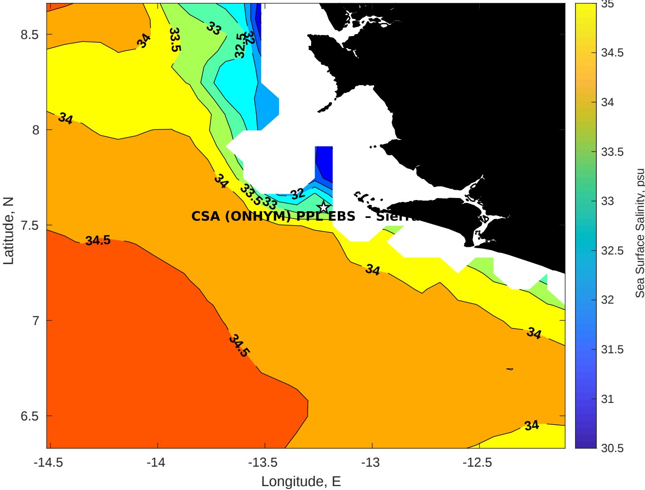
Surface Salinity for CSA (ONHYM) PPL EBS - Sierra Leone at 10-Oct-2025 00:00:00
