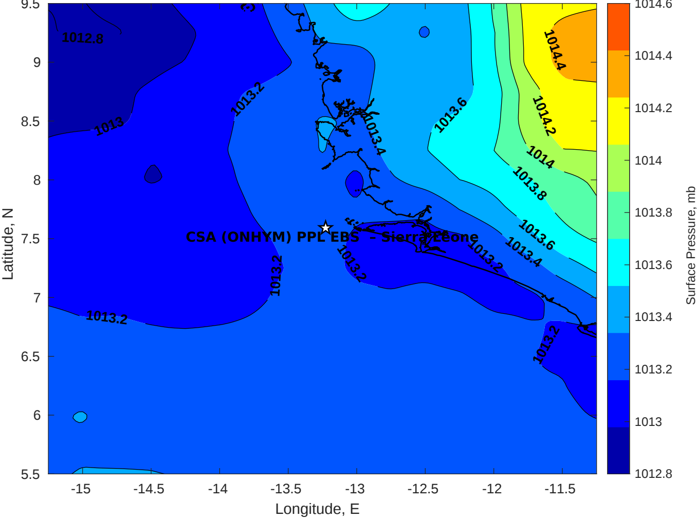
Surface Pressure (mb) for CSA (ONHYM) PPL EBS - Sierra Leone at 11-Oct-2025 00:00:00
