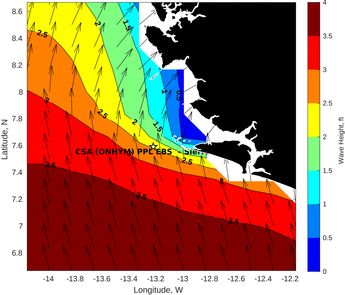
Wave Height (ft) for CSA (ONHYM) PPL EBS - Sierra Leone at 11-Oct-2025 09:00:00
