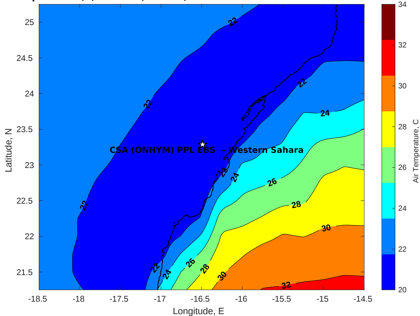
Air Temperature (C) for CSA (ONHYM) PPL EBS - Western Sahara at 11-Oct-2025
