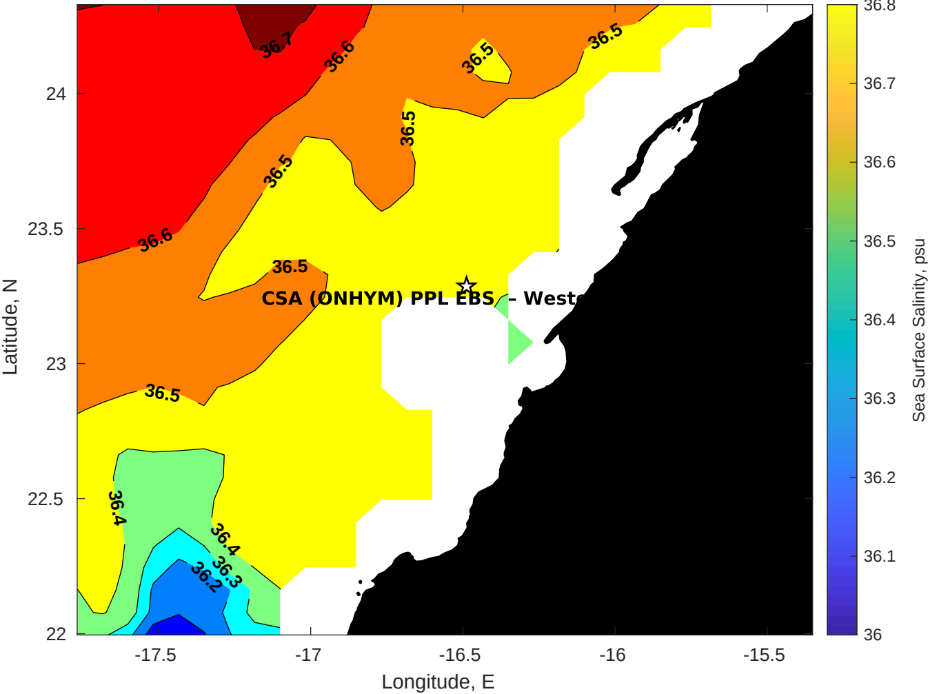
Surface Salinity for CSA (ONHYM) PPL EBS - Western Sahara at 10-Oct-2025 00:00:00
